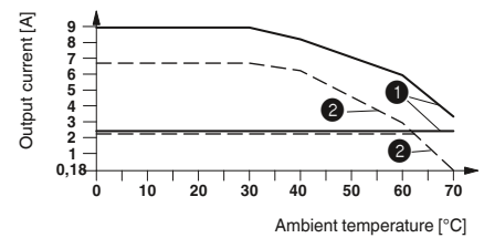
Derating curve ELR H5-IES-SC-24DC/500AC-2 and ELR H5-IES-SC-230AC/500AC-9 100% operating time
