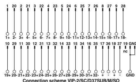
Connection scheme VIP-2/SC/D37SUB/M/SO
