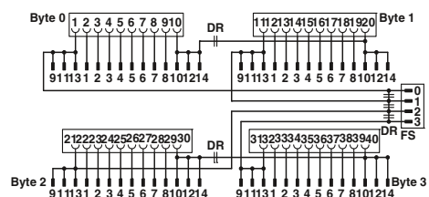
Connection scheme FLKM 50/4-FLK14/PA-S300
