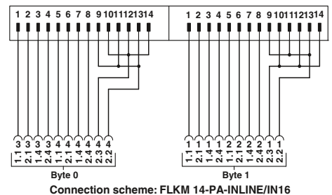
Connection scheme: FLKM 14-PA-INLINE/IN16
