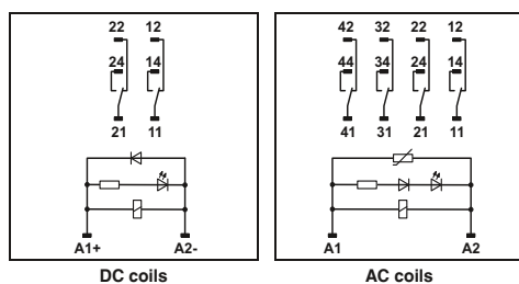
DC coils
