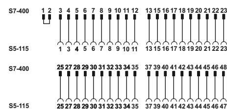
Connection scheme: FLKM S115/S400/SO155
