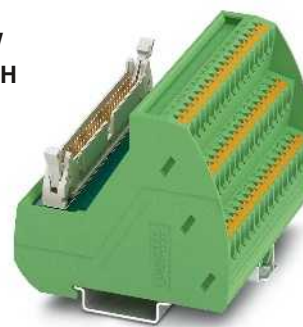
26 to 64 positions with push-in connection and light indicator
