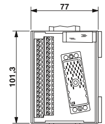
Dimensional drawing for UMK-EC56/32-XUR
