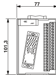
Dimensional drawing for UMK-EC56/32-XUL
