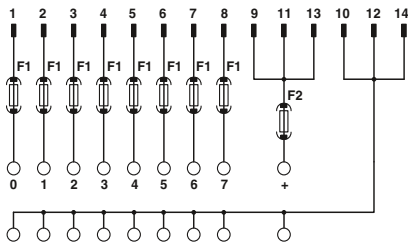
Connection scheme: FLKM 14/8M/SI/PLC
