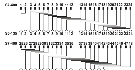
FLKM S135-465-4UA/UI/S400 connection scheme
