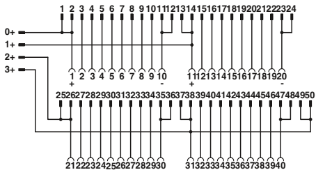
Connection scheme FLKM 50-PA-AB/OBN
