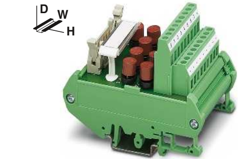
Passive fuse modules for 8 or 32 channels
