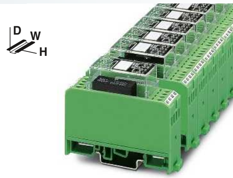
1 PDT, soldered-in relay
