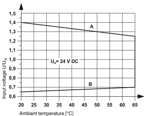
Permissible input voltage range for PLC-BSP-24DC/21RW (with REL-MR-18DC/21... relay)
