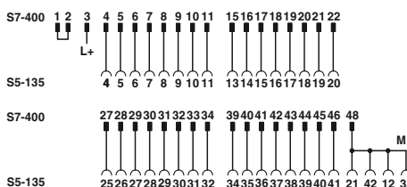
Connection scheme: FLKM S135/S400/SO121
