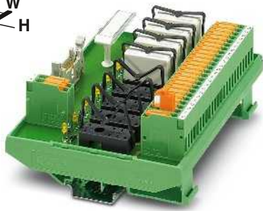
Output module for 8 miniature relays with knife/disconnect terminal blocks, 1 PDT
