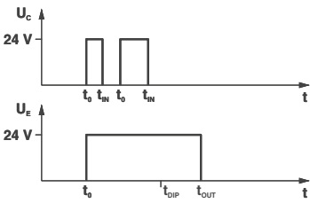
Input pulse t_1 < \text{set output pulse } t_3 (restart when triggered again)
