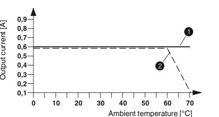
Derating curve ELR H3-I-SC-24DC/500AC-0,6 100% operating time ① Aligned with > 20 mm spacing ② Aligned without spacing
