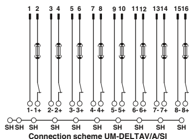
Connection scheme UM-DELTA V/A/SI
