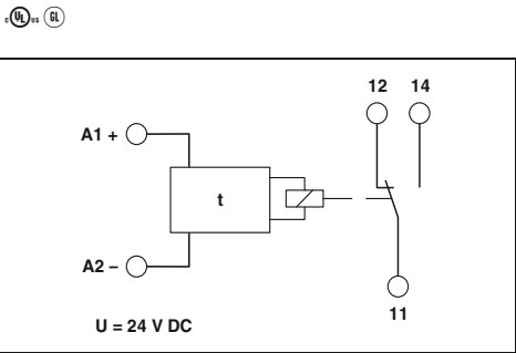
Timer relay with switch-on delay, voltage controlled
