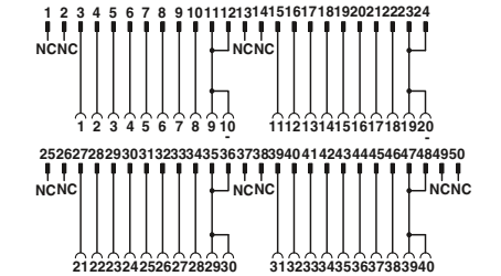
Connection scheme FLKM 50-PA-AB/IBN
