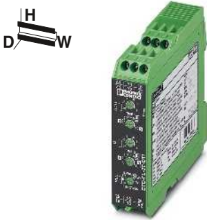
Multifunctional timer relay, two adjustable times
