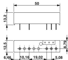
Dimensional drawing for SIM-AMSC:
