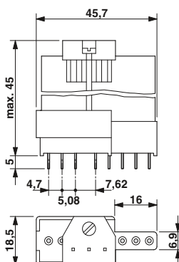
Dimensional drawing for SIM-AMS...R:
