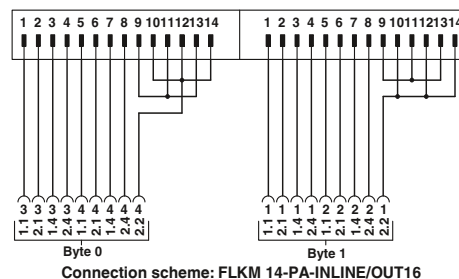
Connection scheme: FLKM 14-PA-INLINE/OUT16
