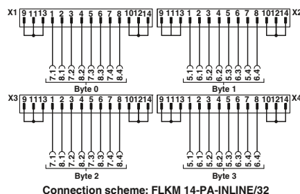
Connection scheme: FLKM 14-PA-INLINE/32
