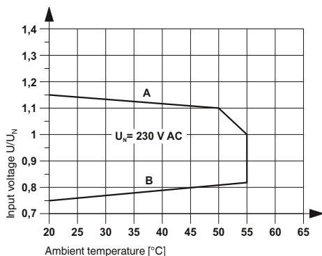
Curve A maximum continuous voltage at limiting continuous current = 6 A
