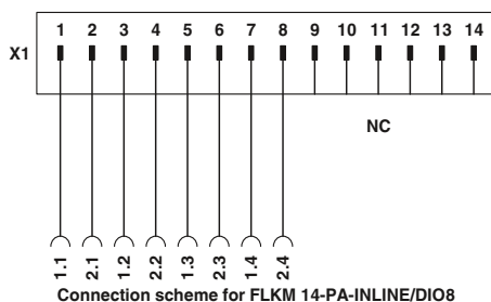
Connection scheme for FLKM 14-PA-INLINE/DIO8
