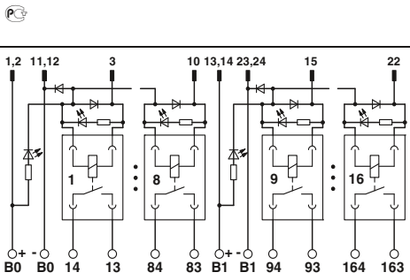
Output base module with 16 miniature relays, 1 N/O contact
