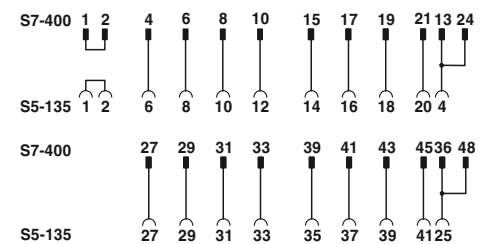
Connection scheme: FLKM S135/S400/SO123
