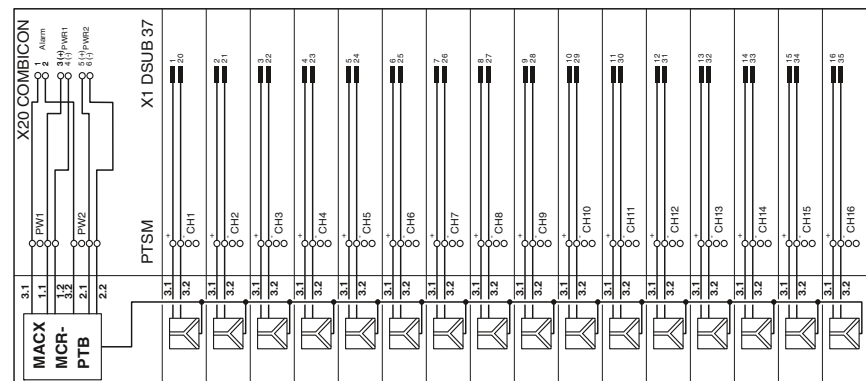
TC-D37SUB-ADIO16-EX-P-UNI and TC-D37SUB-AIO16-EX-PS-UNI connection scheme
