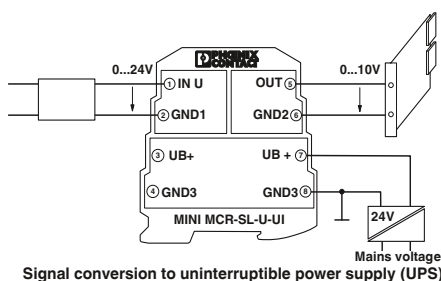
Signal conversion to uninterruptible power supply (UPS)
