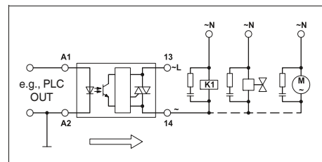
Example: switching the contactor, solenoid valve or motor (AC load)
