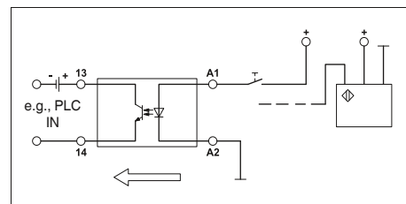
Example: position indication with limit stop contact or initiator
