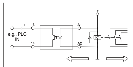
Example: load contactor monitoring (AC contactor)
