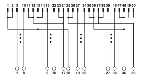
Connection scheme VIP-2/.../FLK50/AB-1756
