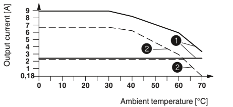
Derating curve ELR H3-I-SC-24DC/500AC-2 and ELR H3-I-SC-24DC/500AC-9 100% operating time
