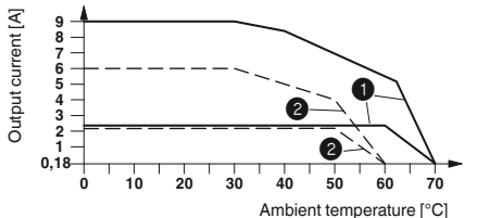
Derating curve ELR H3-I-SC-230AC/500AC-2 and ELR H3-I-SC-230AC/500AC-9 100% operating time
