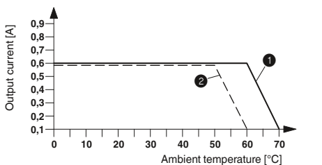
Derating curve ELR H3-I-SC-230AC/500AC-0,6 100% operating time
