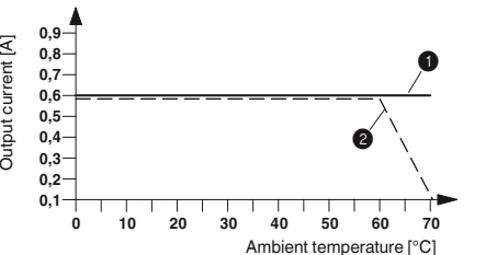
Derating curve ELR H3-I-SC-24DC/500AC-0,6 100% operating time
