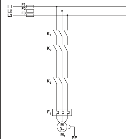
Conventional structure Main current path contactor according to category 3
