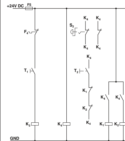
Conventional structure Control current path contactor according to category 3
