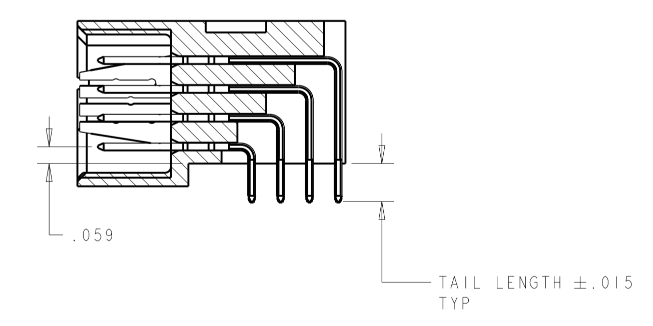
SECTION Z-Z
