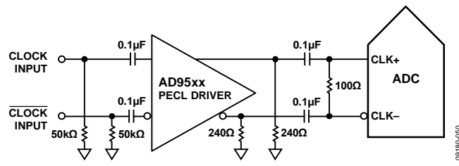
Figure 56. Differential PECL Sample Clock (Up to 640 MHz)
