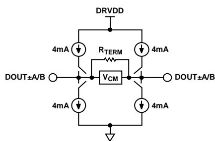
Figure 43. Digital CML Output
