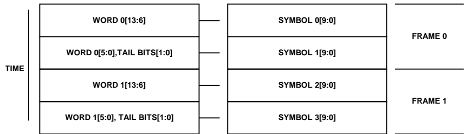
Figure 64. AD9644 14-Bit Data Transmission with Tail Bits
