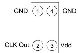
Figure 2. Pin Assignments (CSP)
