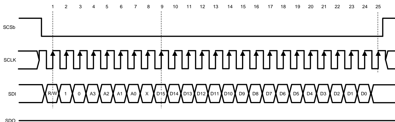
Figure 69. Serial Data Protocol - Write Operation
