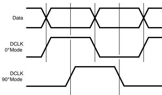
Figure 70. DDR DCLK-to-Data Phase Relationship
