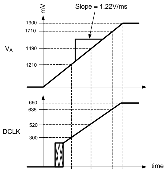
Figure 81. Supply and DCLK Ramping
