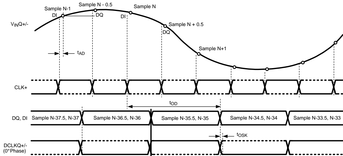
Figure 10. Clocking in Non-Demux Mode DES Mode*
