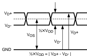
Figure 5. LVDS Output Signal Levels
