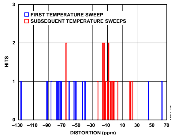
Figure 67. Thermal Hysteresis
