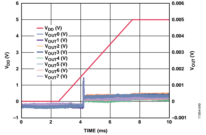
Figure 42. Power-On Reset to 0 V and Midscale
