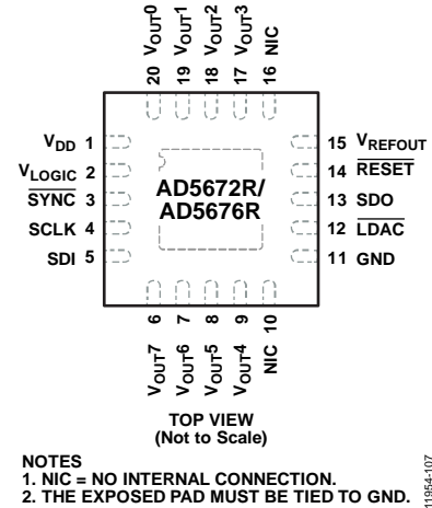
Figure 7. LFCSP Pin Configuration
