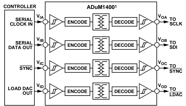
Figure 72. Isolated Interface
