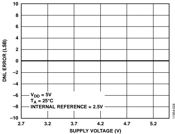
Figure 22. AD5672R DNL Error vs. Supply Voltage
