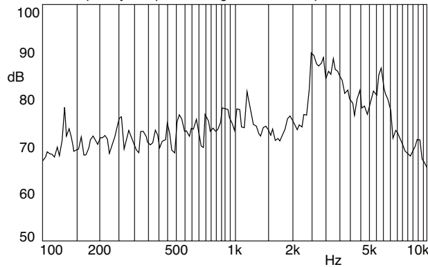
x:2.7384kHz Y:86.94dB ZA: Live Curve SSR T. RMS A: Frequency Response, Magn dB re 20.00 \mu PA
