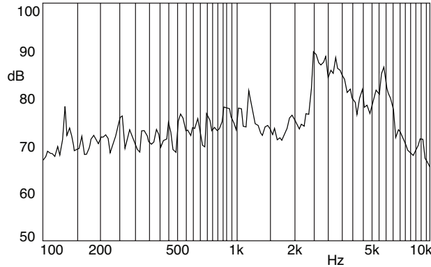
x:2.7384kHz Y:86.94dB ZA: Live Curve SSR T. RMS A: Frequency Response, Magn dB re 20.00 \mu PA
