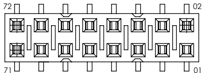
FIGURE 7 POLARIZING POSITIONS
