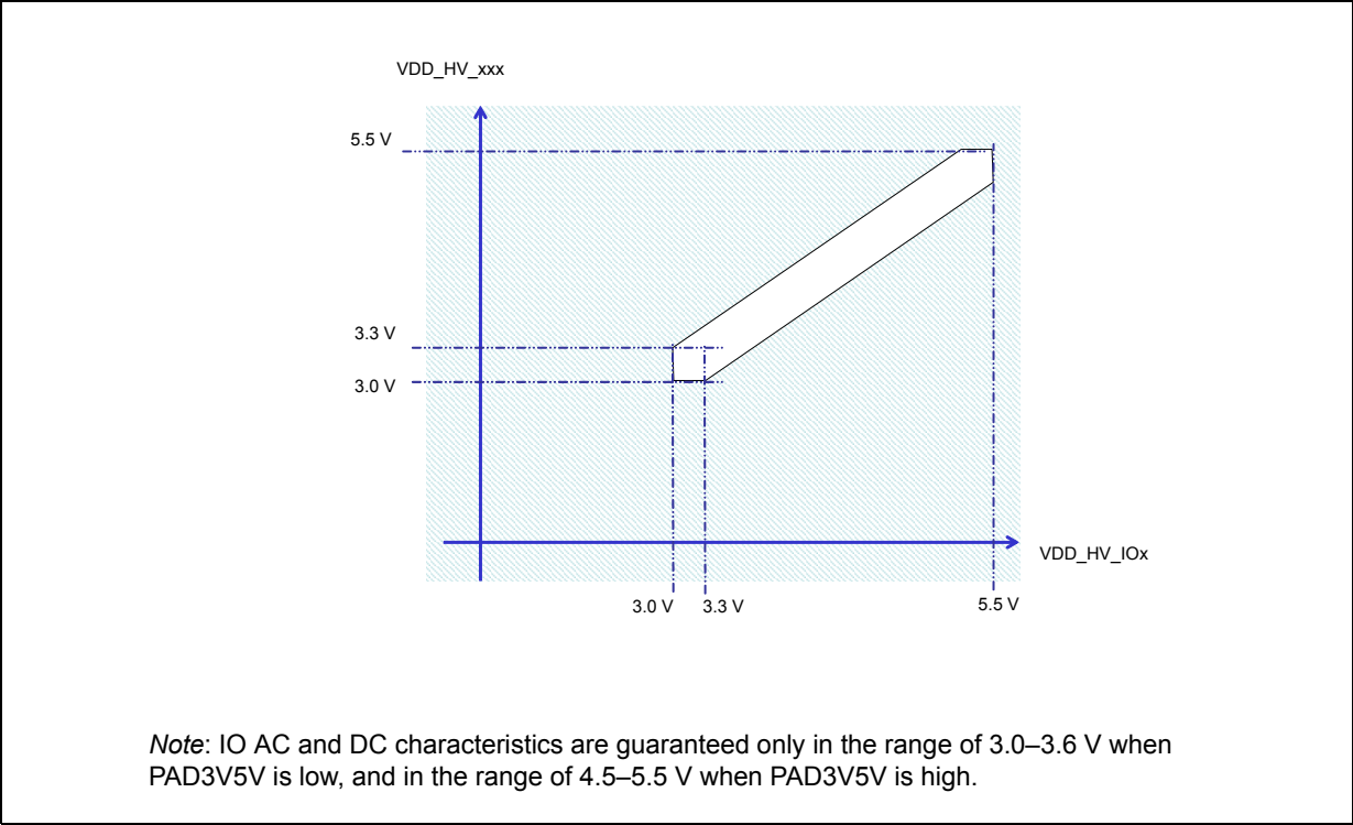
Figure 6. Power supplies constraints (3.0 V ≤ VDD_HV_IOx ≤ 5.5 V)
