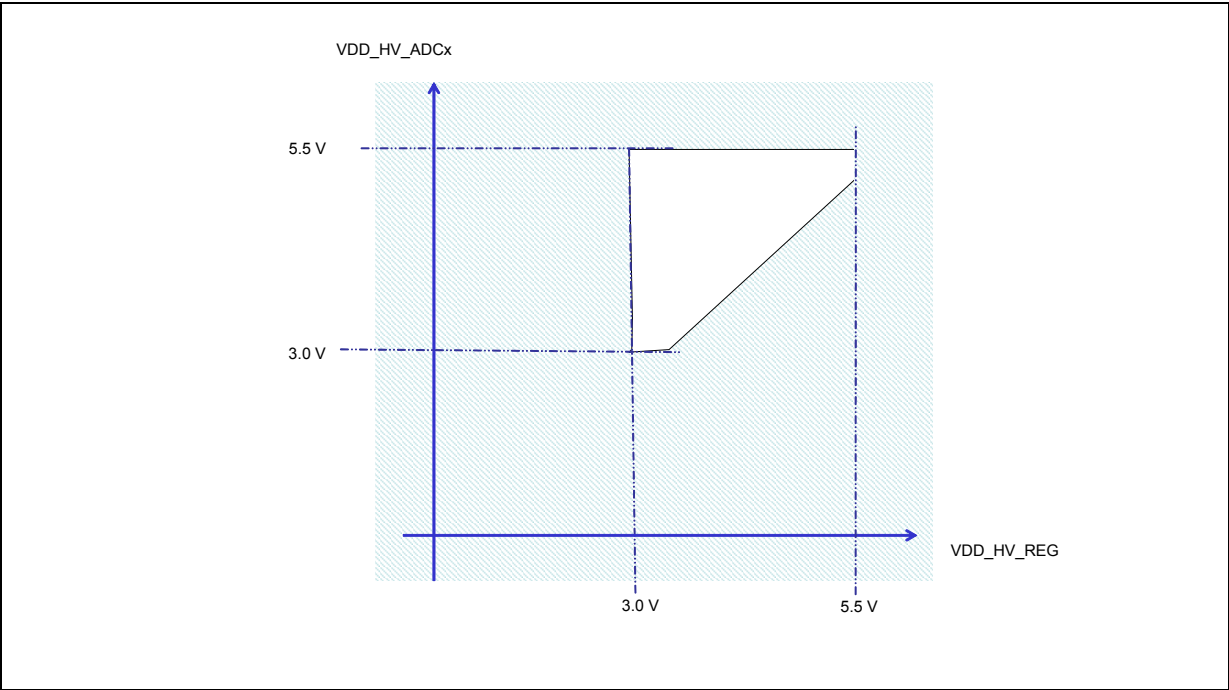
Figure 7. Independent ADC supply (3.0 V ≤ VDD_HV_REG ≤ 5.5 V)
