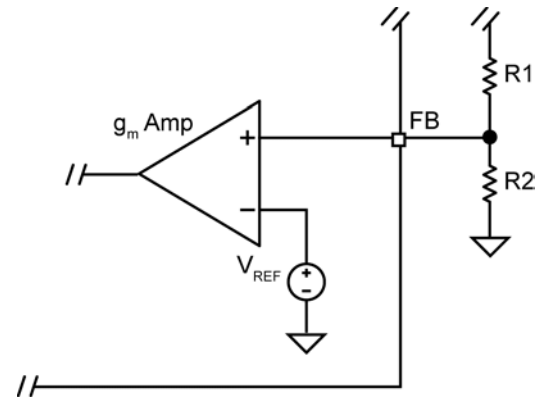
Figure 7. Voltage-Divider Configuration
