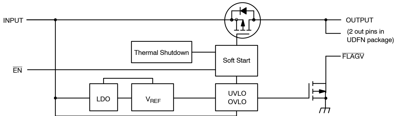
Figure 2. Functional Block Diagram
