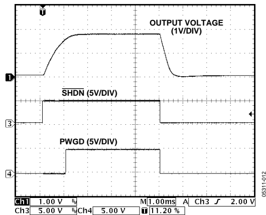
Figure 11. Power-On Response
