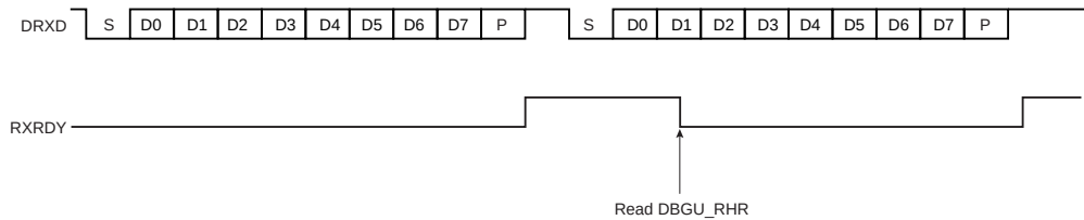
Figure 41-6. Receiver Ready
