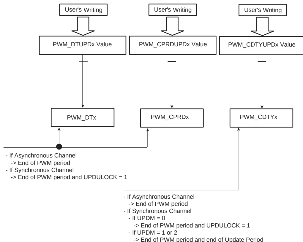
Figure 46-19. Synchronized Period, Duty-Cycle and Dead-Time Update
