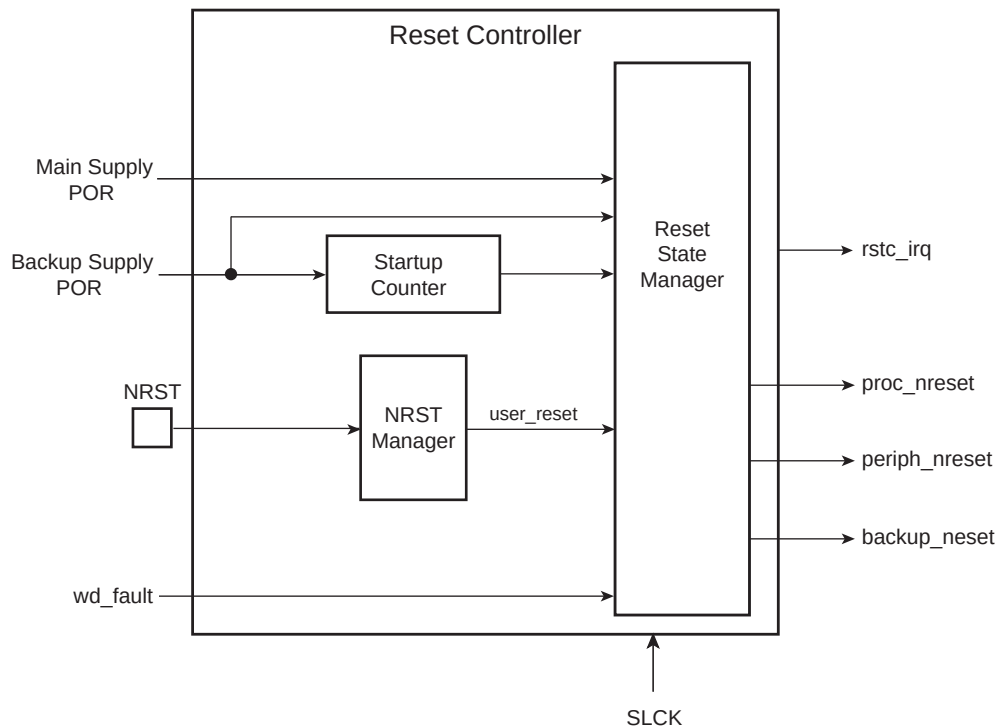
Figure 19-1. Reset Controller Block Diagram
