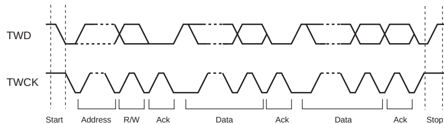
Figure 39-3. Transfer Format
