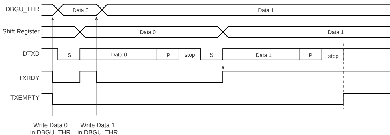
Figure 41-11. Transmitter Control
