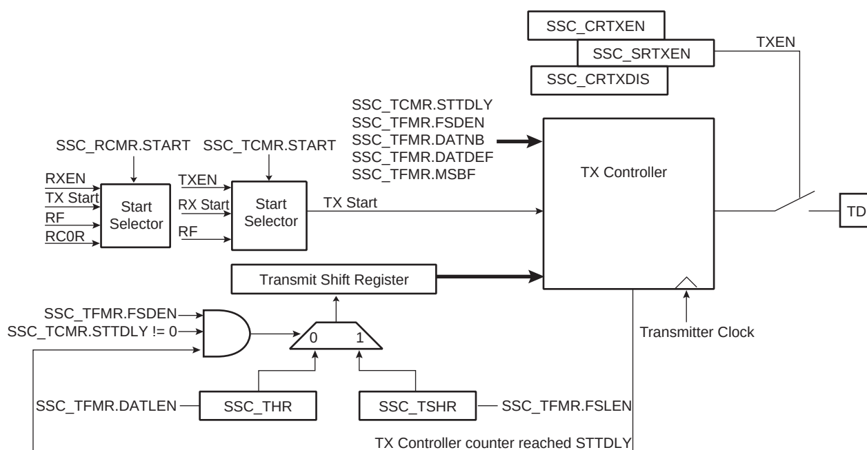
Figure 40-11. Transmitter Block Diagram
