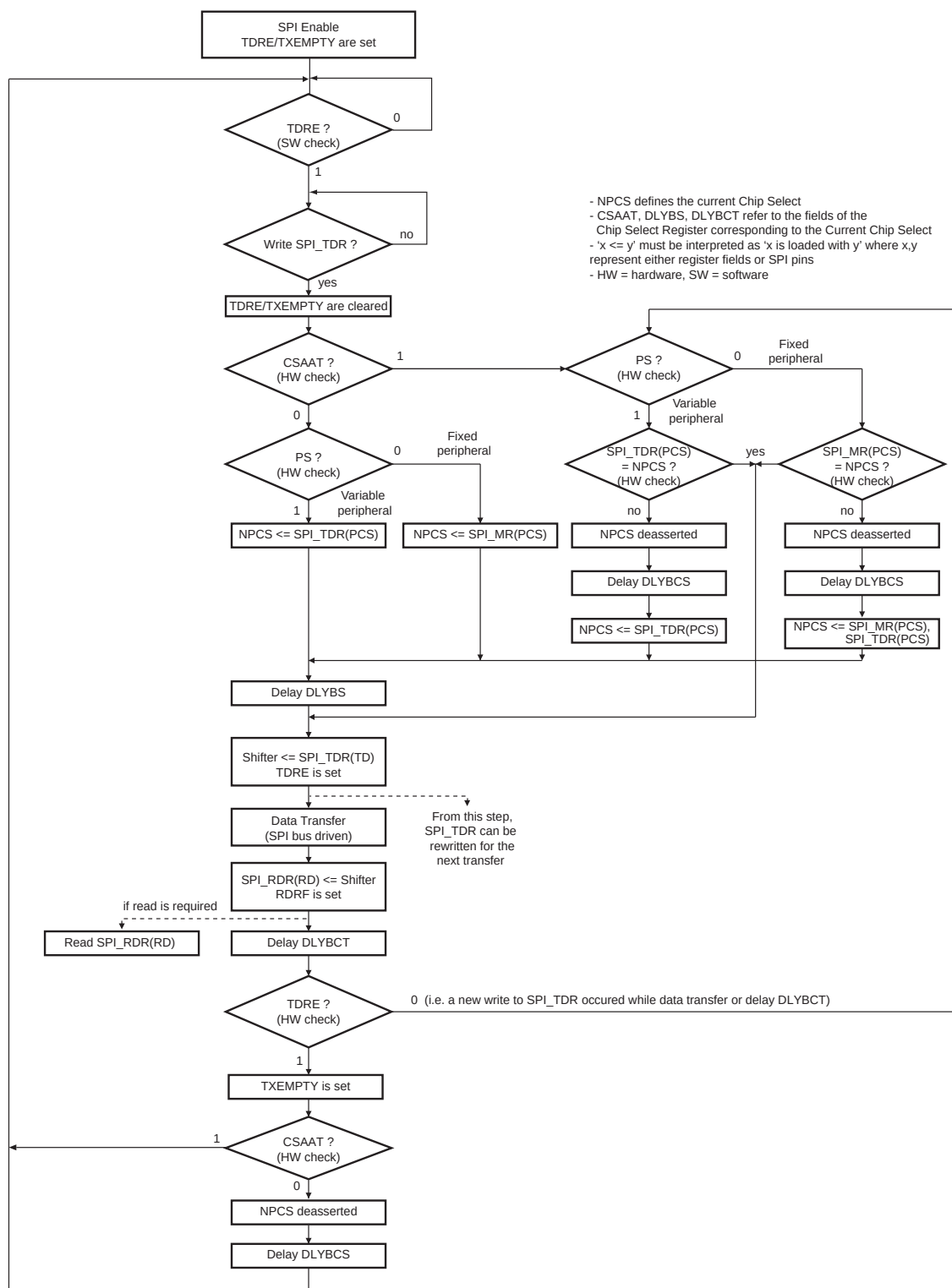
Figure 38-7. Master Mode Flow Diagram
