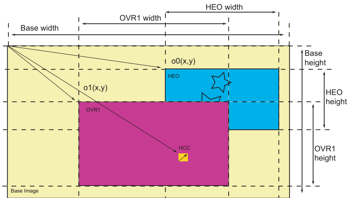
Figure 31-9. Overlay Example with Two Different Video Prioritization Algorithms
