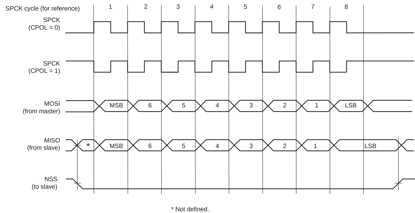
Figure 38-4. SPI Transfer Format (NCPHA = 0, 8 bits per transfer)
