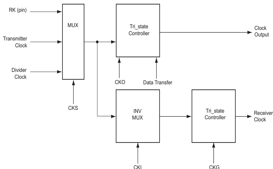
Figure 40-10. Receiver Clock Management
