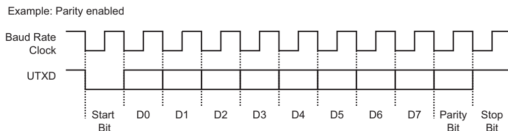
Figure 42-9. Character Transmission
