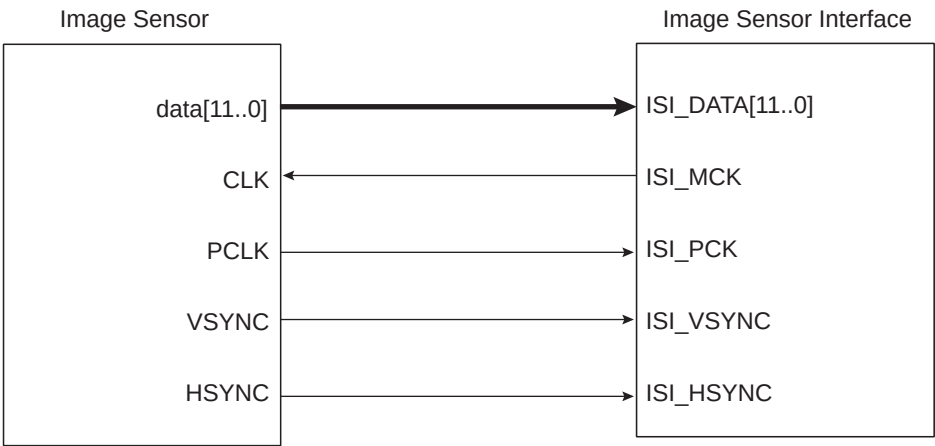
Figure 33-1. ISI Connection Example
