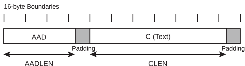
Figure 49-6. Full Message Alignment
