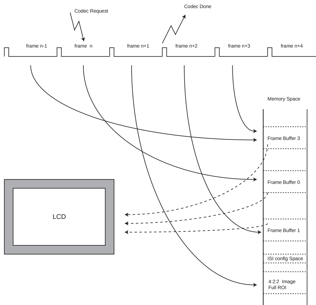
Figure 33-6. Three Frame Buffers Application and Memory Mapping
