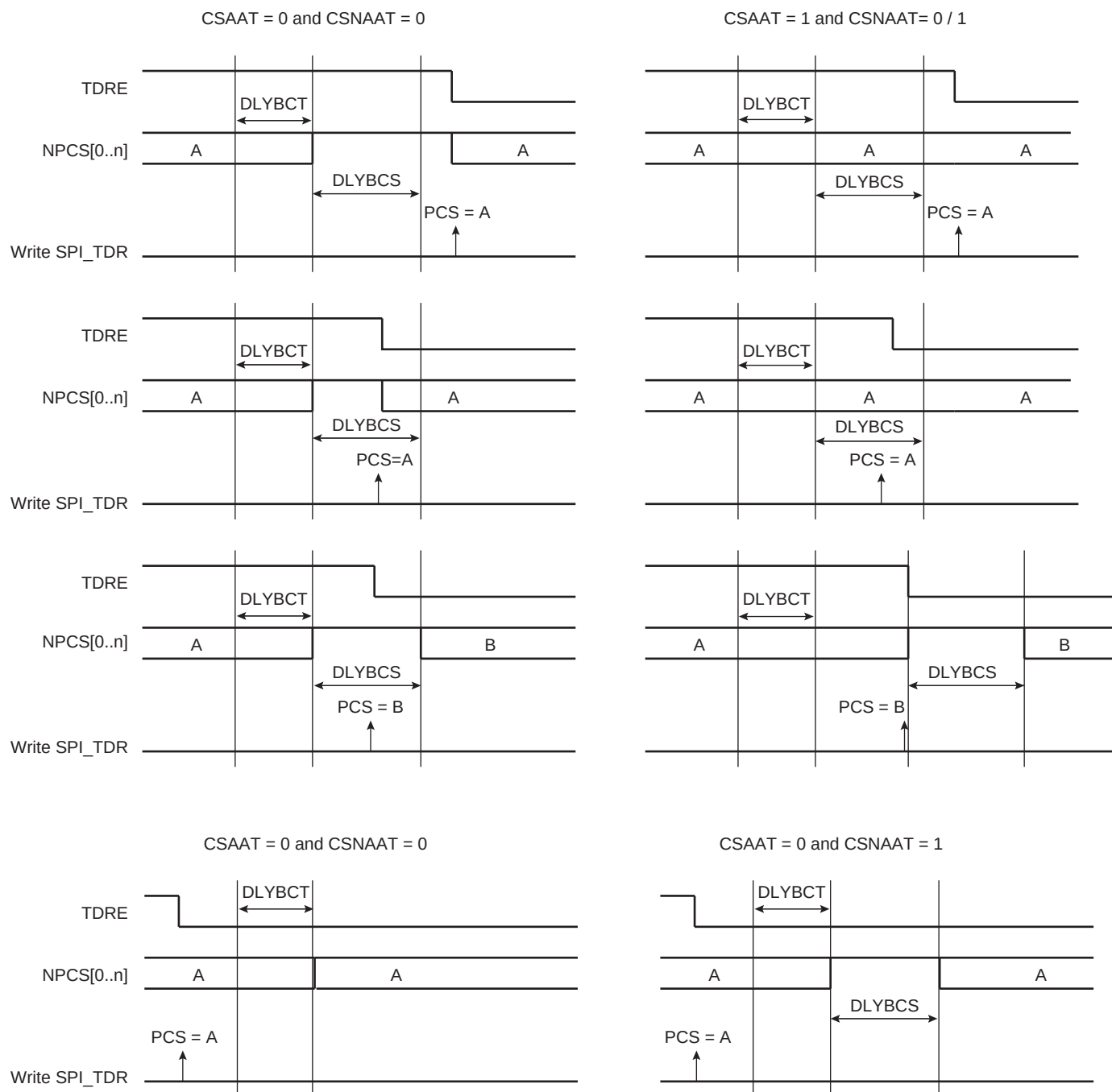
Figure 38-11. Peripheral Deselection
