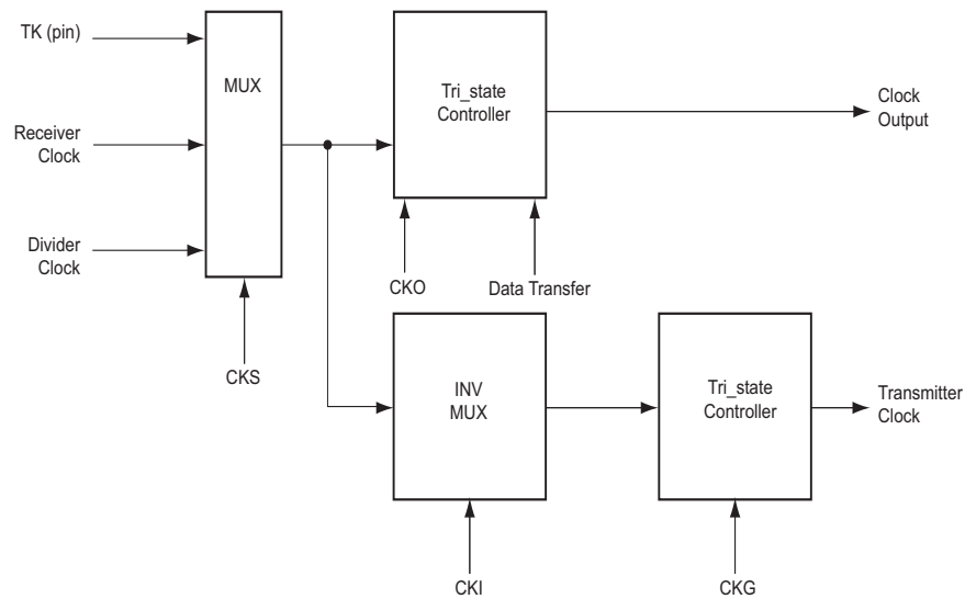
Figure 40-9. Transmitter Clock Management
