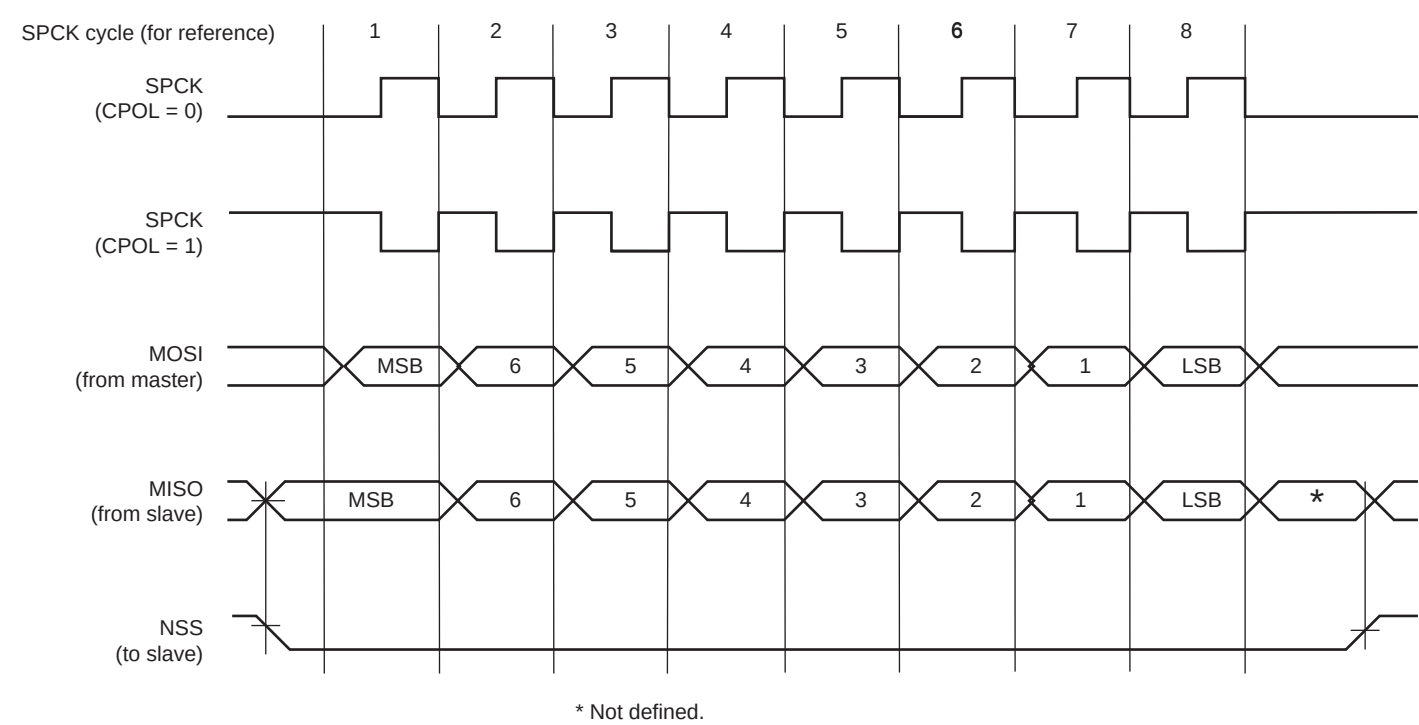
Figure 38-3. SPI Transfer Format (NCPHA = 1, 8 bits per transfer)
