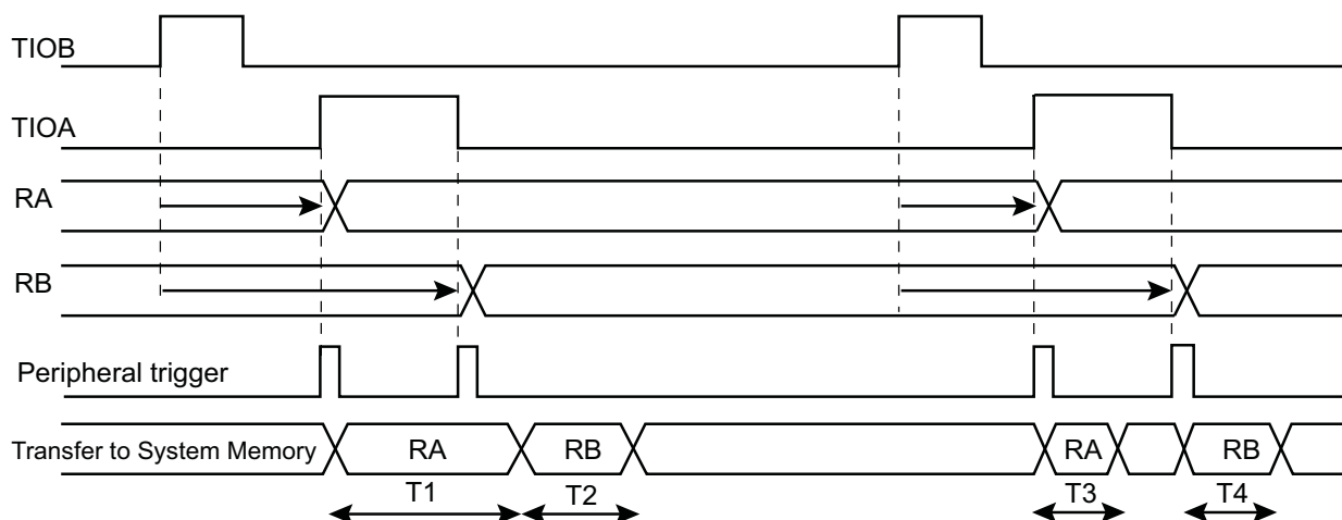
Figure 45-5. Example of Transfer with DMAC
