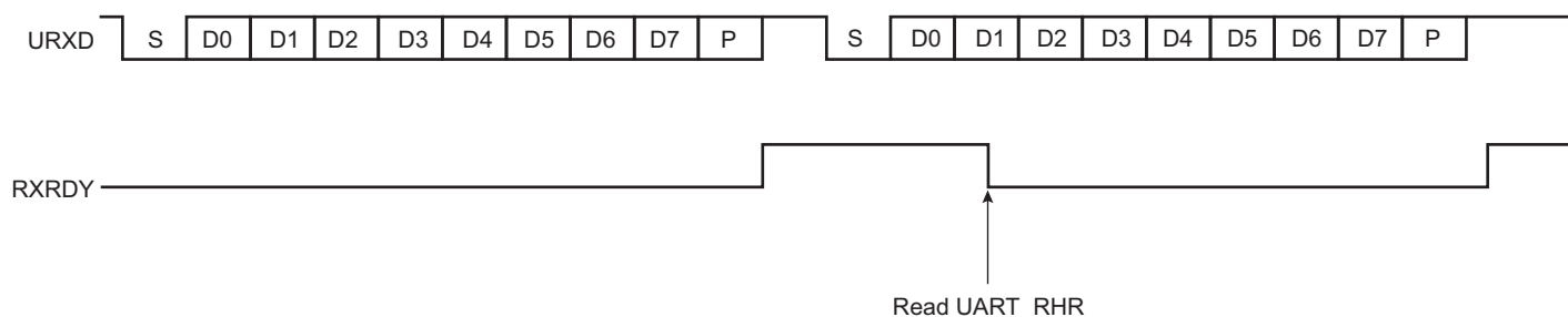
Figure 42-5. Receiver Ready
