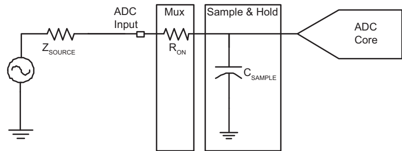
Figure 55-2. Simplified Acquisition Path
