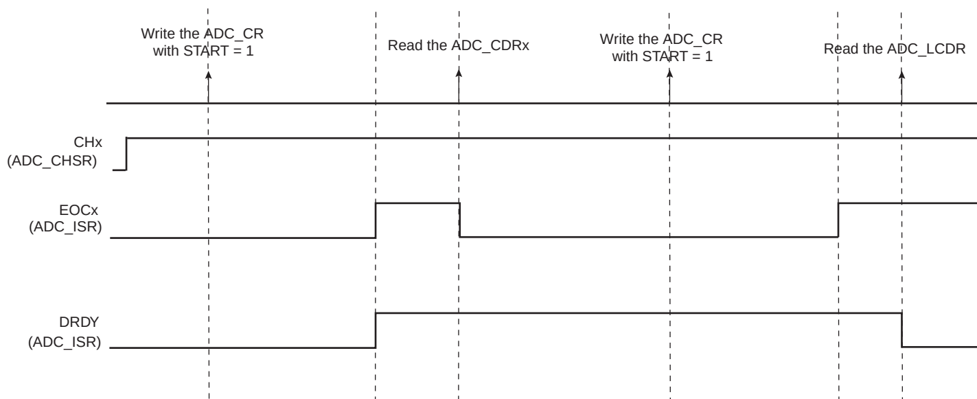
Figure 47-3. EOCx and DRDY Flag Behavior
