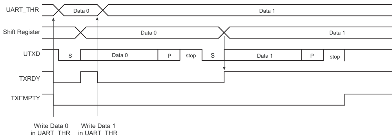
Figure 42-10. Transmitter Control
