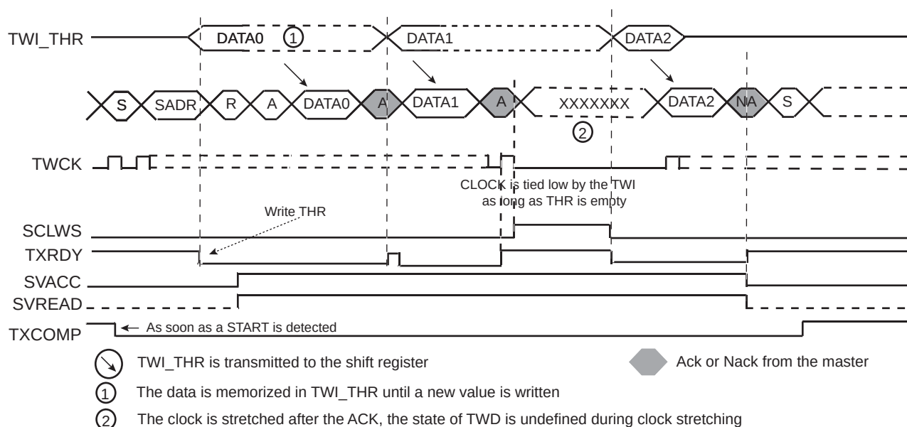
Figure 39-25. Clock Stretching in Read Mode
