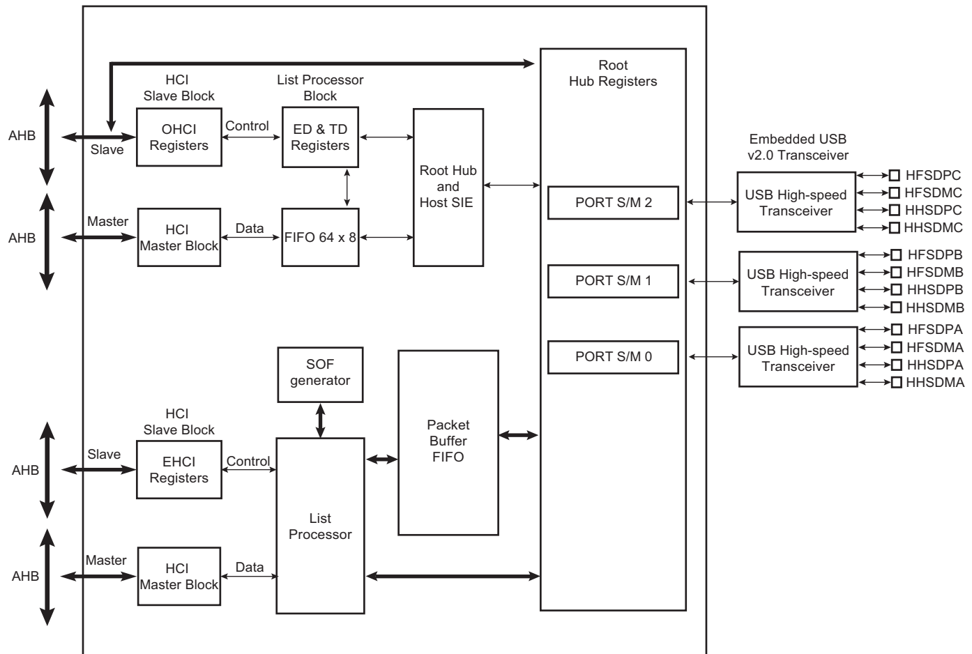
Figure 35-1. Block Diagram
