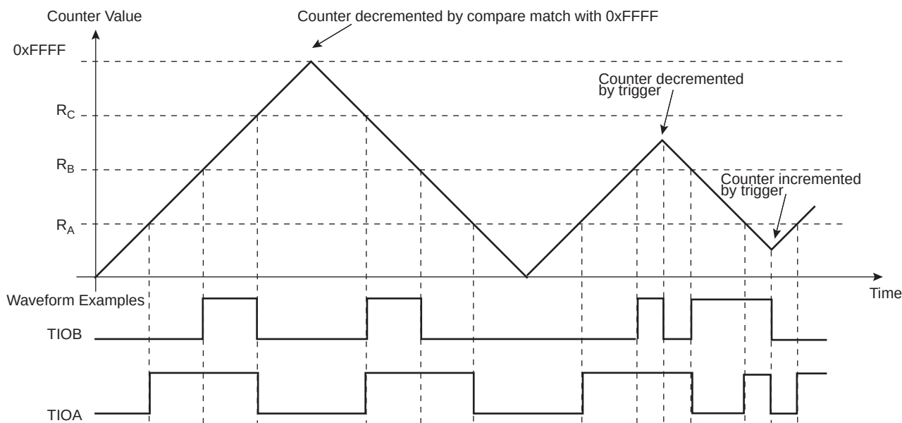
Figure 45-13. WAVSEL = 01 with Trigger
