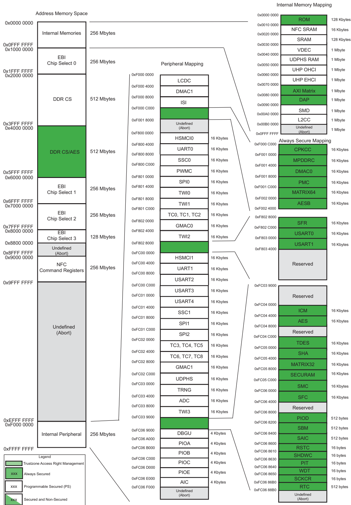
Figure 5-1. SAMA5D4 Series Memory Mapping
