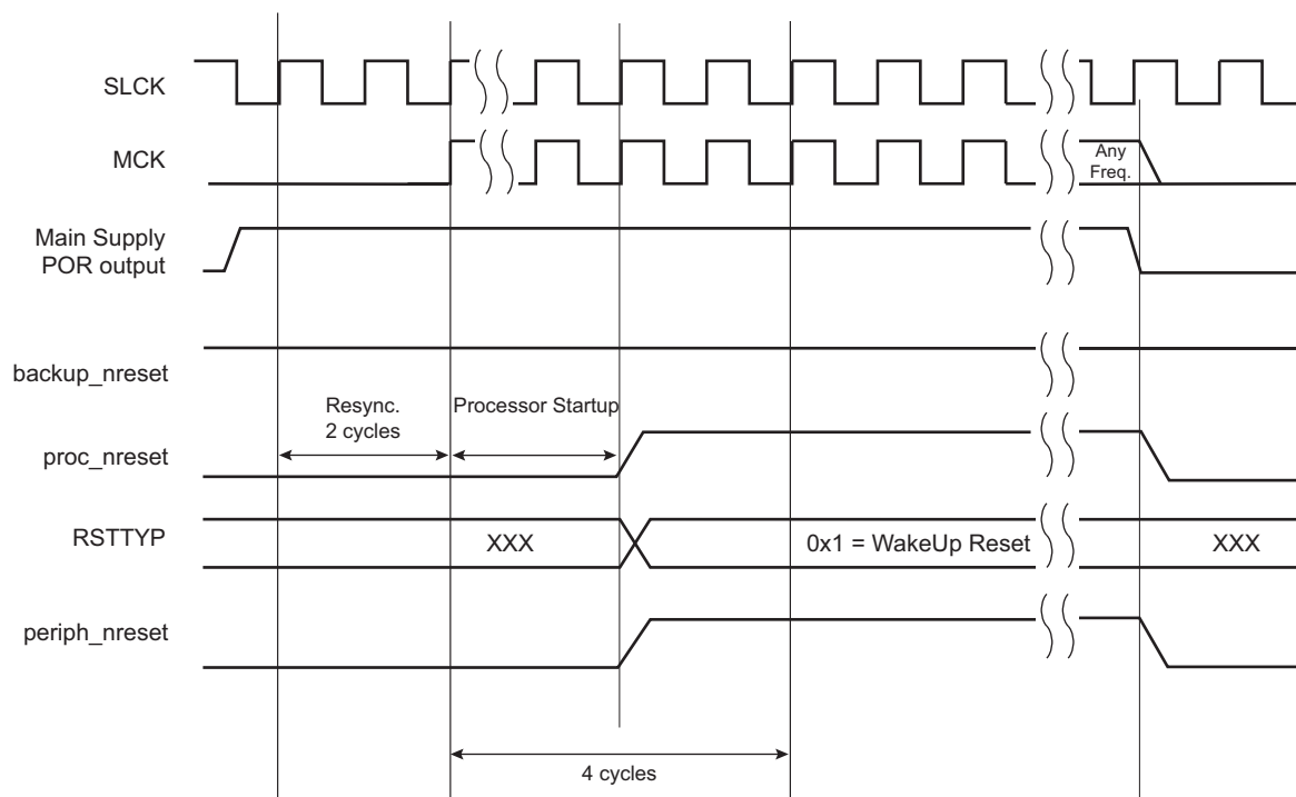
Figure 19-4. Wake-up Reset
