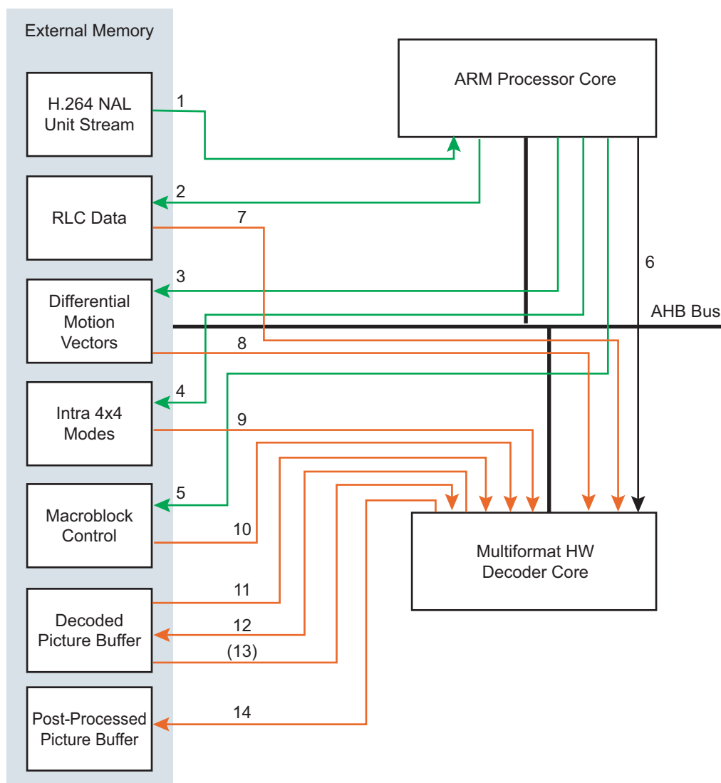
Figure 32-3. Multi-format Decoder and External Memory Data Flow in RLC Mode
