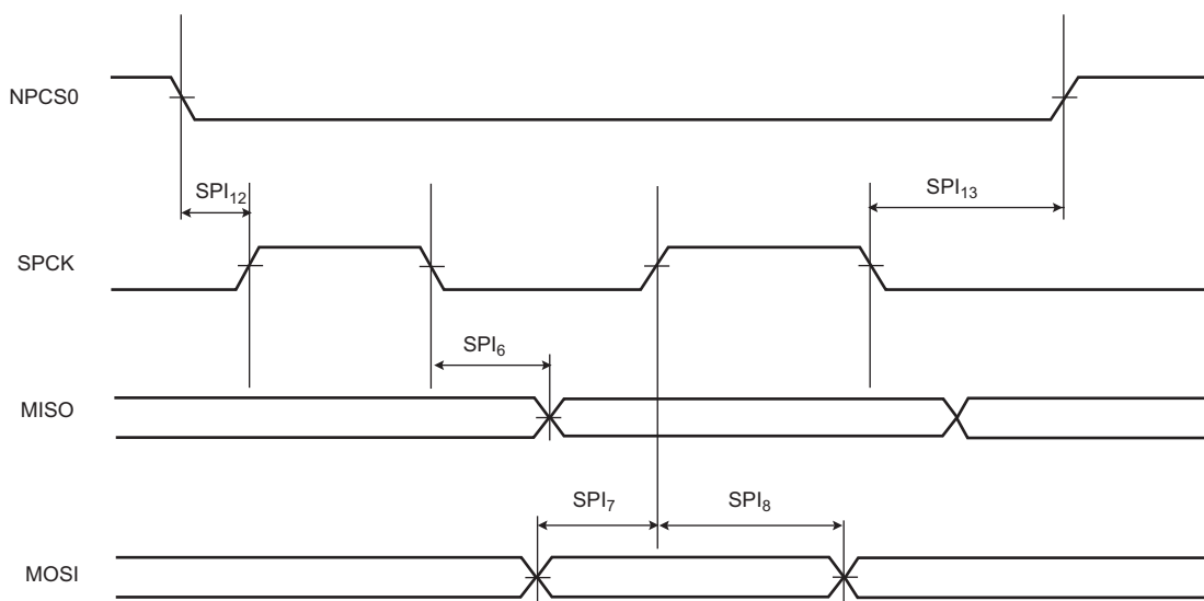
Figure 55-8. SPI Slave Mode 0 and 3
