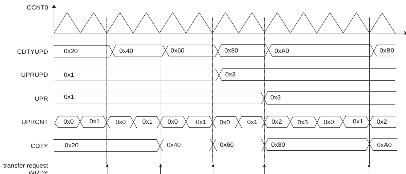
Figure 46-13. Method 3 (UPDM = 2 and PTRM = 0)
