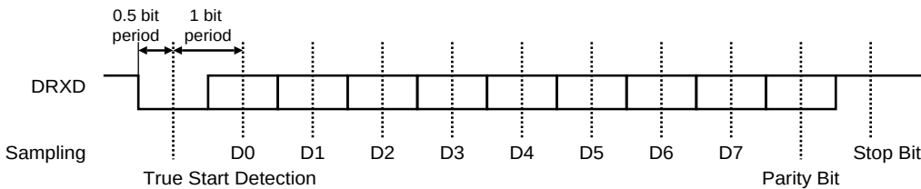
Figure 41-5. Character Reception
