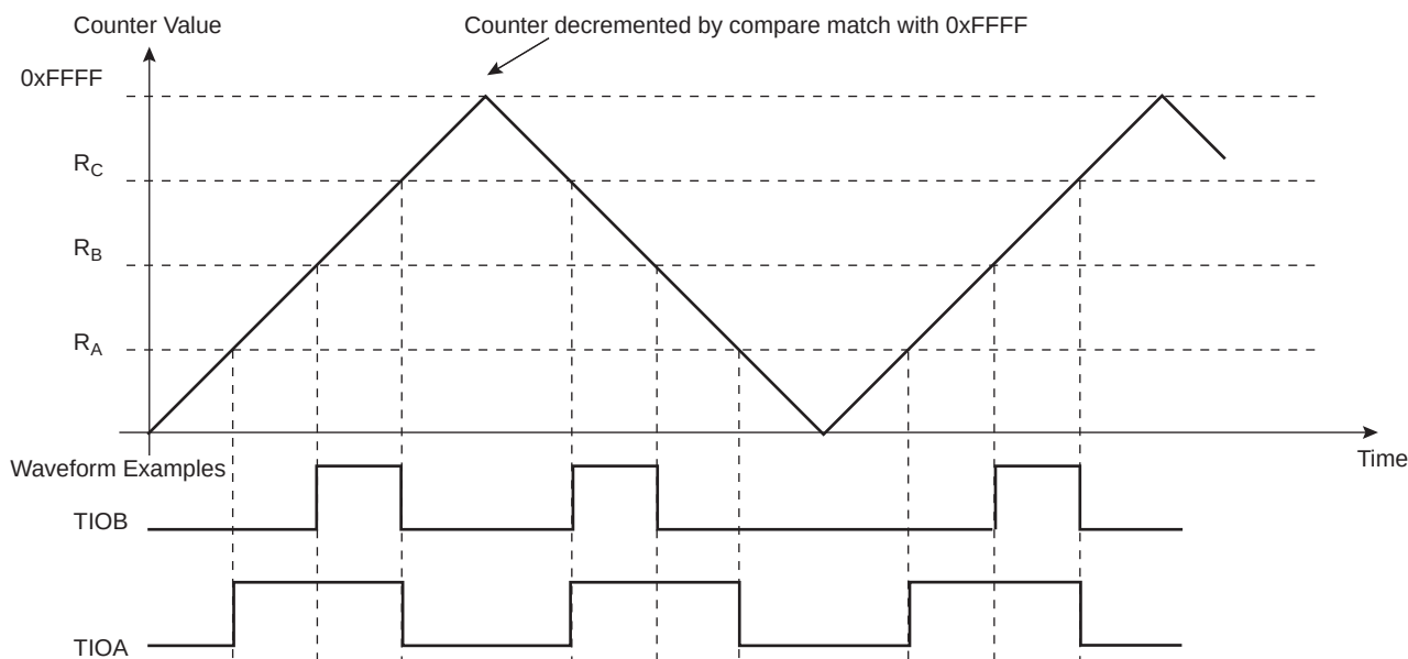
Figure 45-12. WAVSEL = 01 without Trigger
