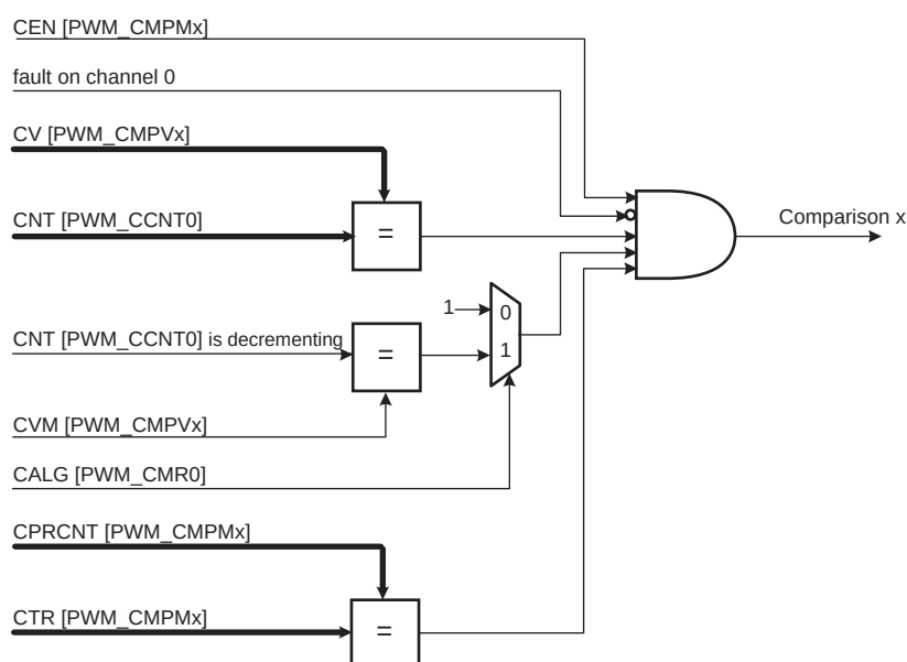
Figure 46-15. Comparison Unit Block Diagram
