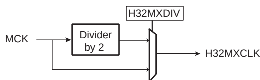
Figure 26-3. H32MX 32-bit Matrix Clock Configuration
