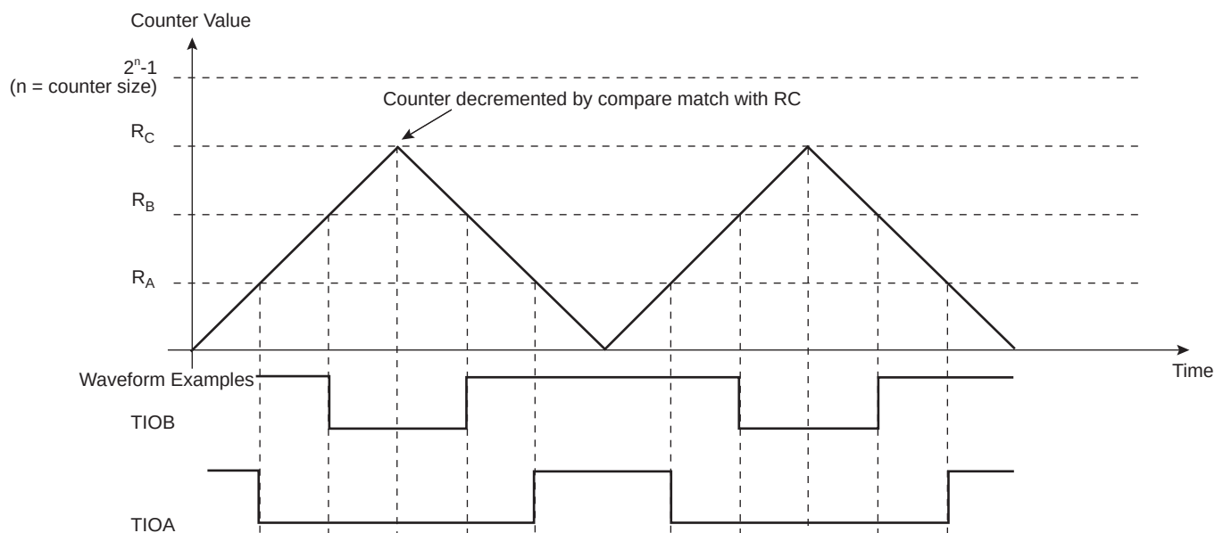
Figure 45-14. WAVSEL = 11 without Trigger
