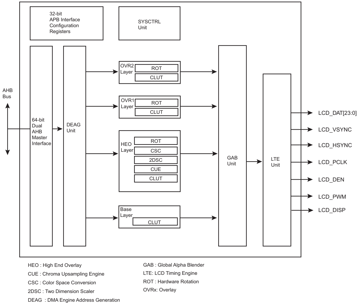
Figure 31-1. Block Diagram
