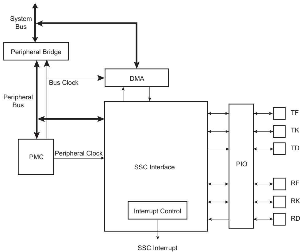
Figure 40-1. Block Diagram
