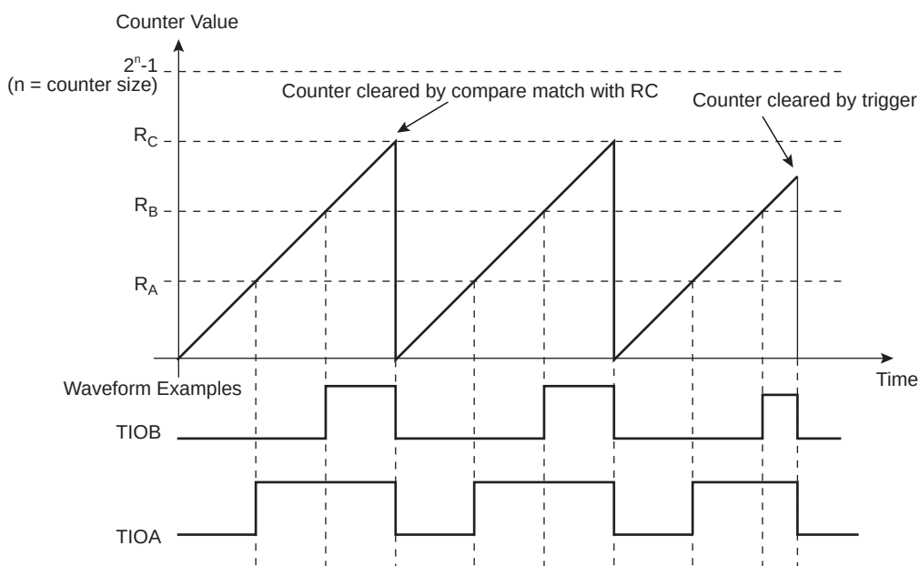
Figure 45-11. WAVSEL = 10 with Trigger
