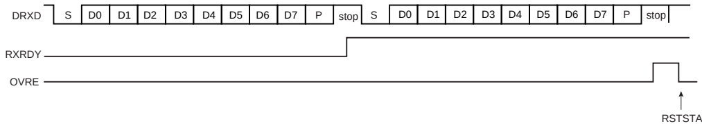
Figure 41-7. Receiver Overrun
