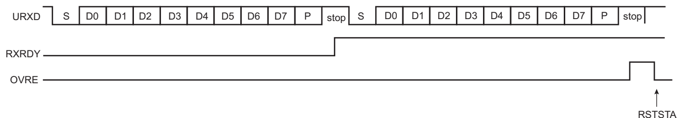
Figure 42-6. Receiver Overrun
