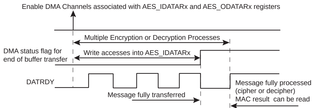
Figure 49-4. DMA Transfer with AES_MR.LOD = 1
