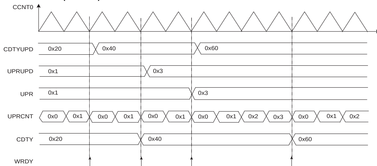
Figure 46-12. Method 2 (UPDM = 1)
