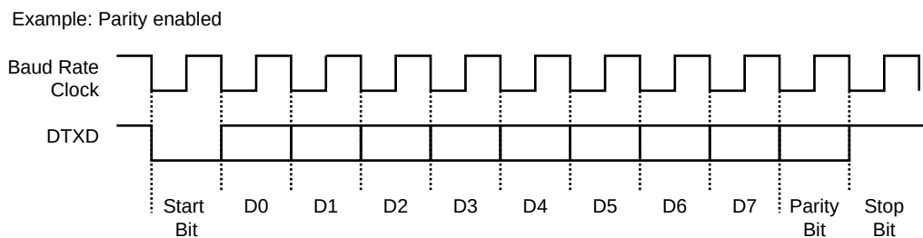
Figure 41-10. Character Transmission
