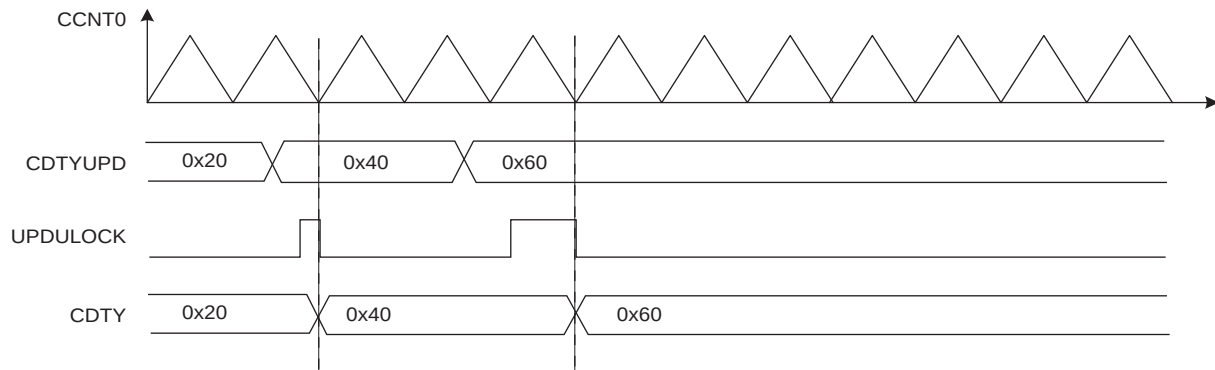
Figure 46-11. Method 1 (UPDM = 0)
