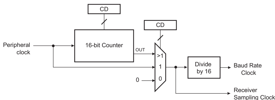
Figure 41-3. Baud Rate Generator
