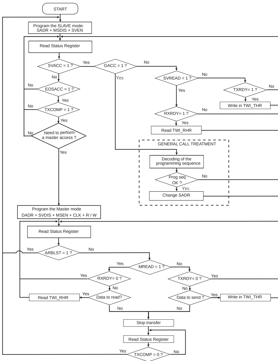
Figure 39-21. Multi-master Flowchart
