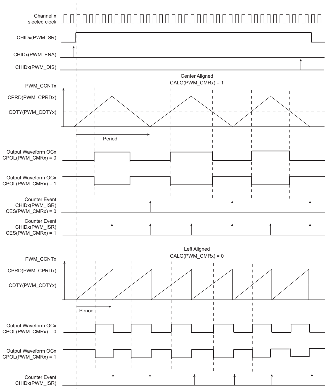
Figure 46-5. Waveform Properties
