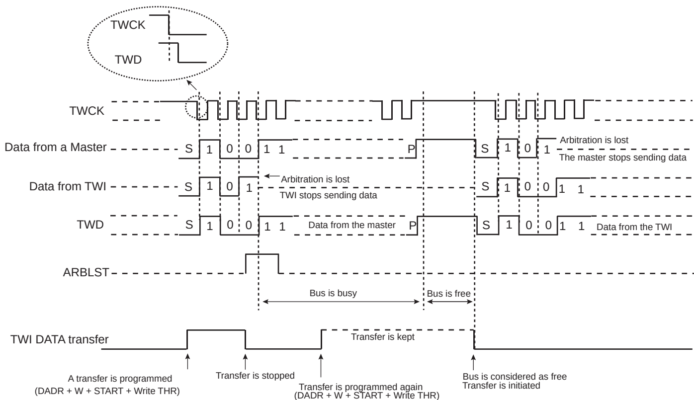
Figure 39-20. Arbitration Cases
