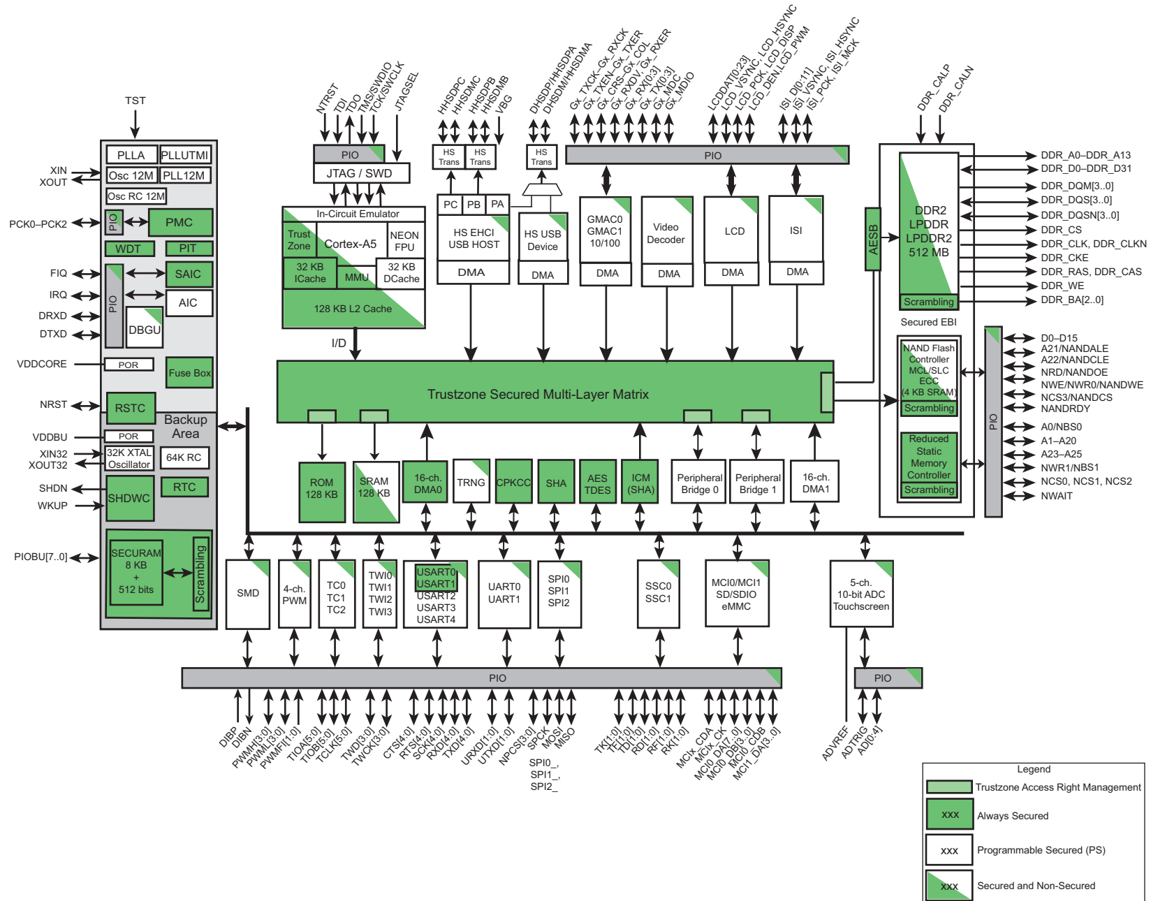
Figure 1-1. SAMA5D4 Series Block Diagram
