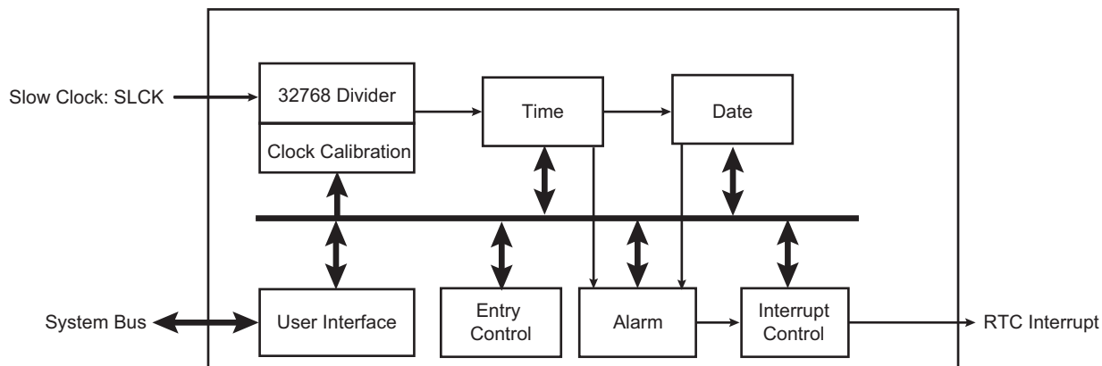
Figure 22-1. Real-time Clock Block Diagram
