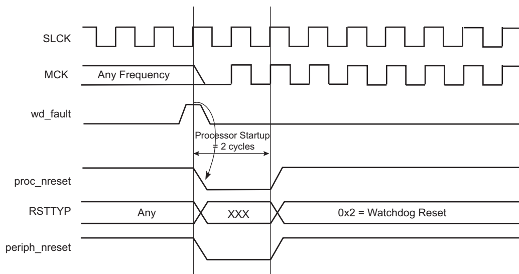
Figure 19-7. Watchdog Reset
