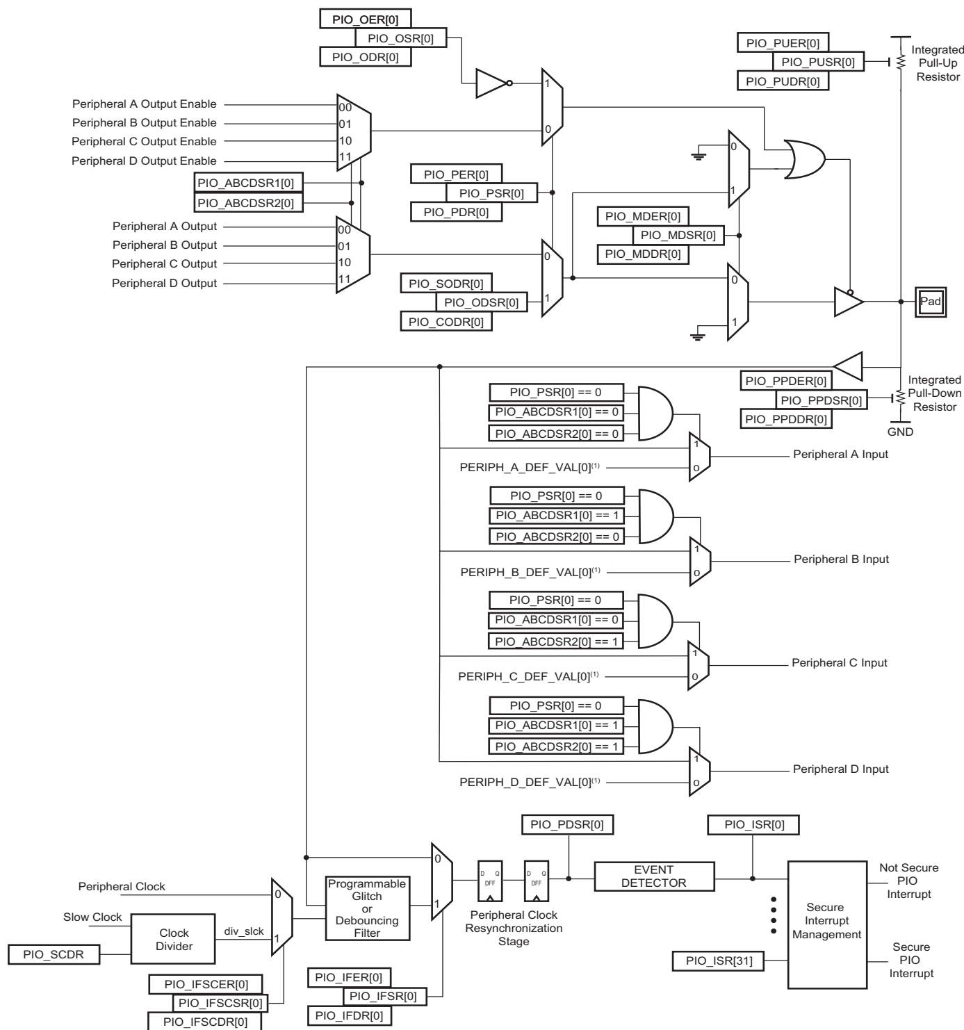
Figure 27-2. I/O Line Control Logic
