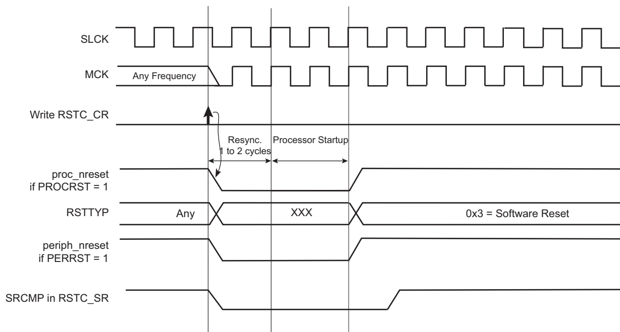
Figure 19-6. Software Reset
