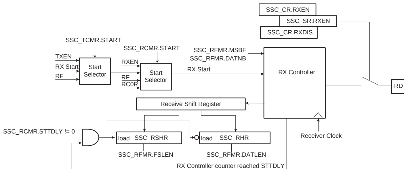
Figure 40-12. Receiver Block Diagram
