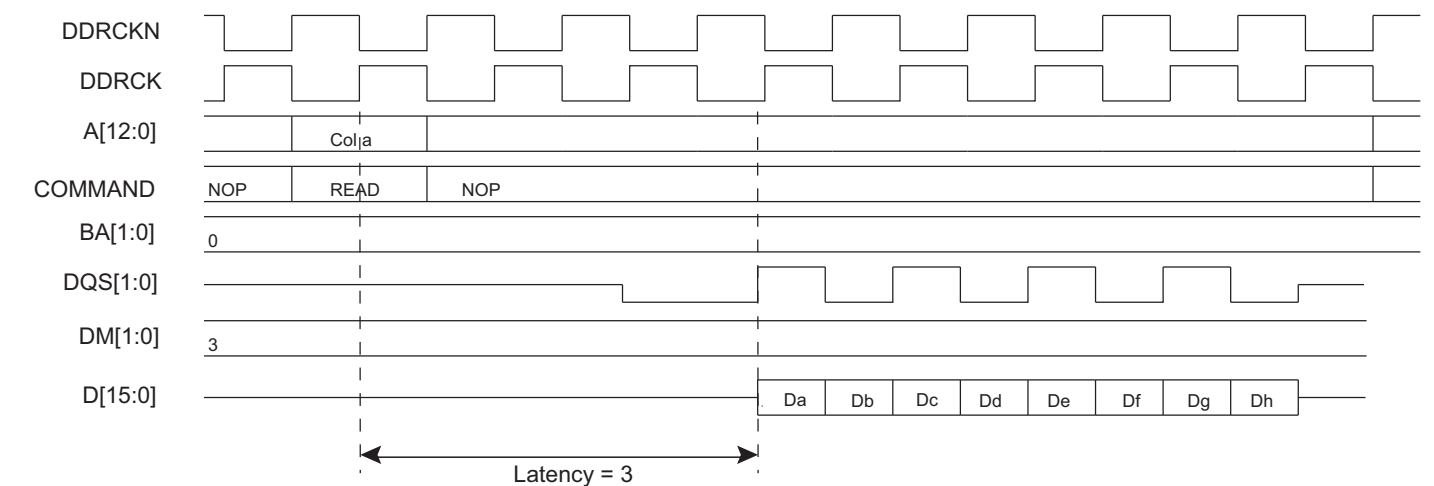
Figure 28-12. Burst Read Access, Latency = 3, DDR2-SDRAM Devices
