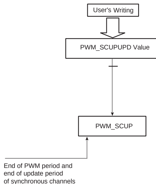
Figure 46-20. Synchronized Update of Update Period Value of Synchronous Channels
