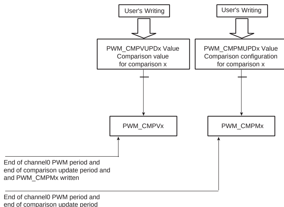
Figure 46-21. Synchronized Update of Comparison Values and Configurations
