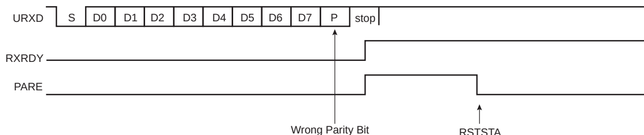
Figure 42-7. Parity Error
