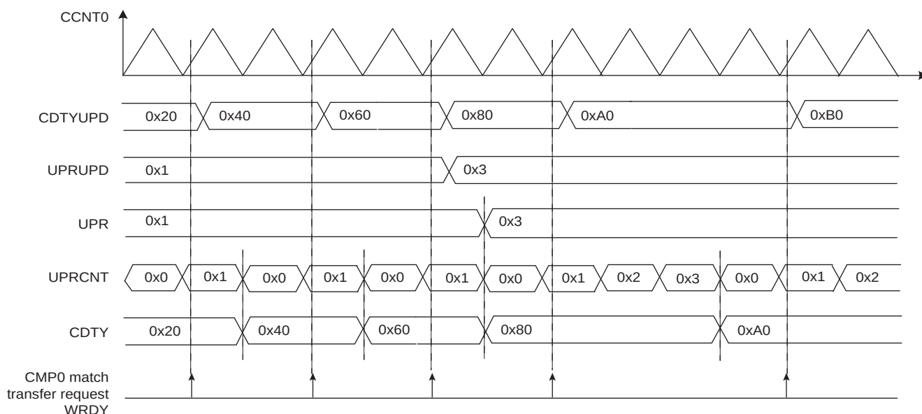
Figure 46-14. Method 3 (UPDM = 2 and PTRM = 1 and PTRCS = 0)
