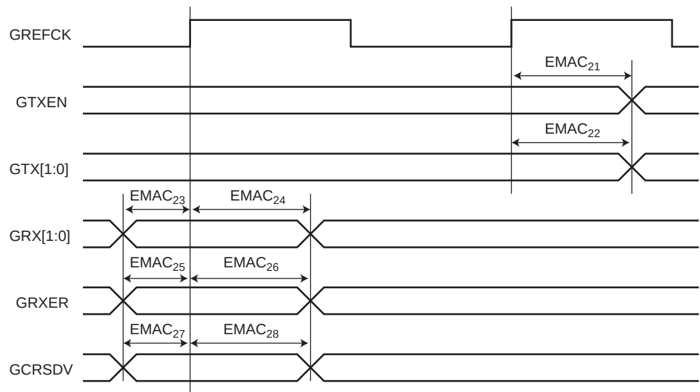
Figure 55-25. Ethernet MAC RMII Timings
