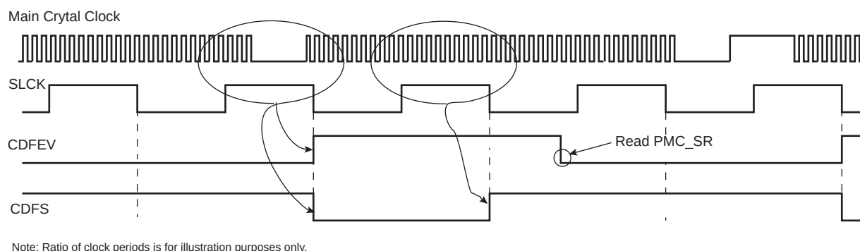
Figure 26-6. Clock Failure Detection (Example)
