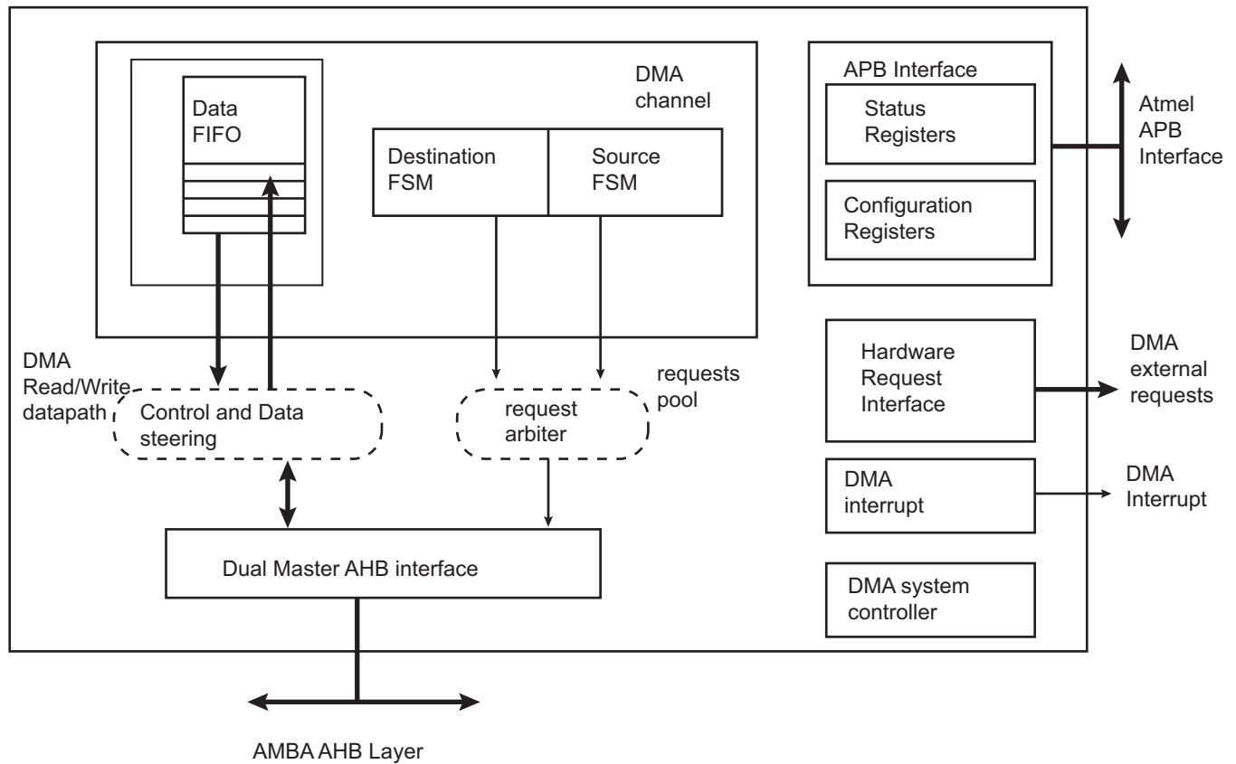
Figure 30-1. DMA Controller (XDMAC) Block Diagram
