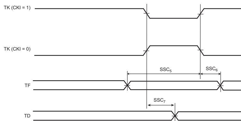
Figure 55-16. SSC Transmitter, TK and TF in Input
