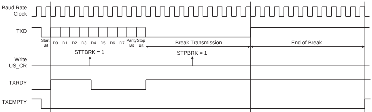
Figure 43-25. Break Transmission
