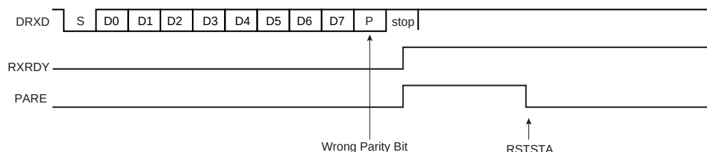
Figure 41-8. Parity Error
