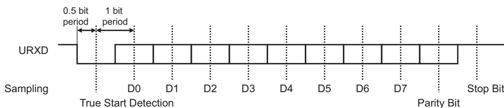
Figure 42-4. Character Reception
