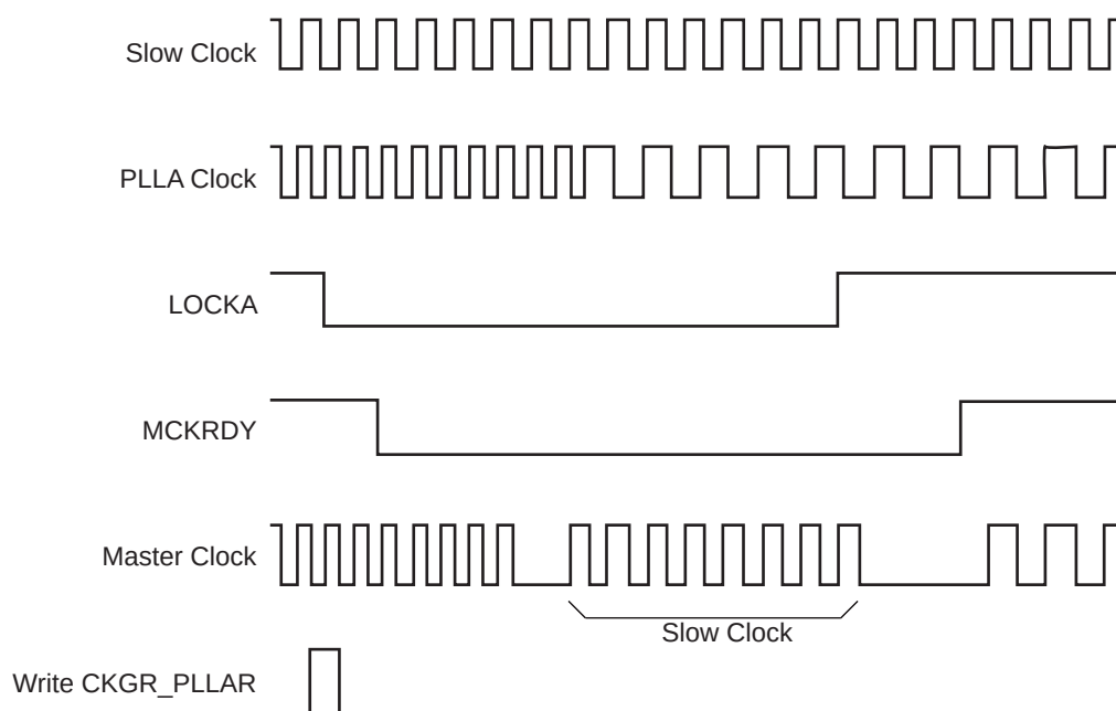
Figure 26-9. Change PLLA Programming
