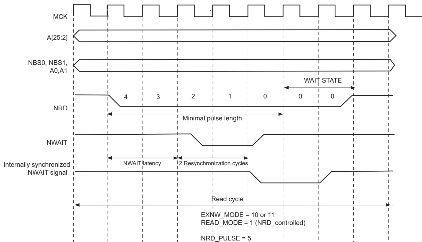
Figure 29-27. NWAIT Latency
