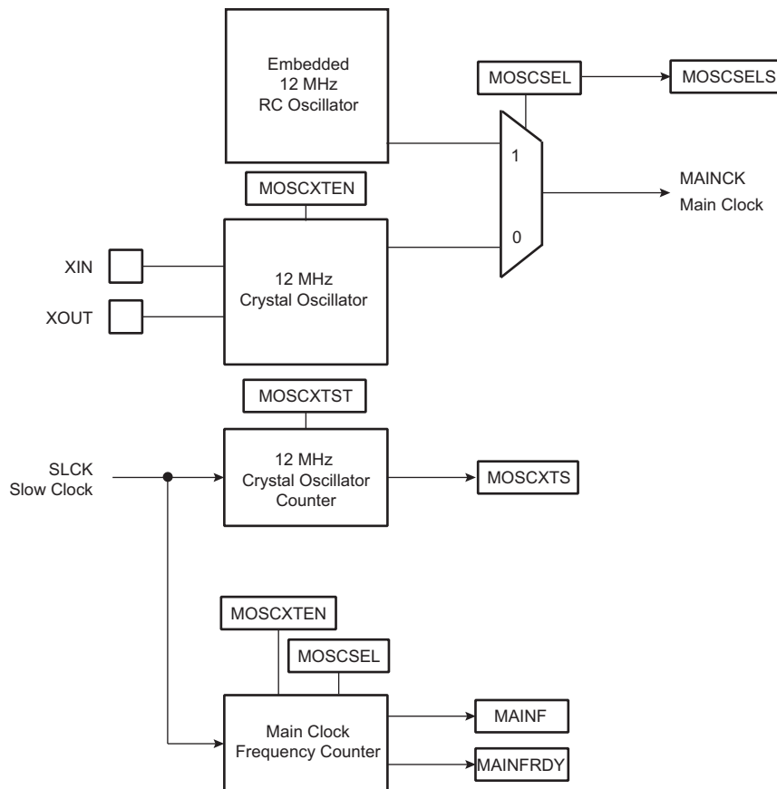
Figure 25-3. Main Clock Block Diagram
