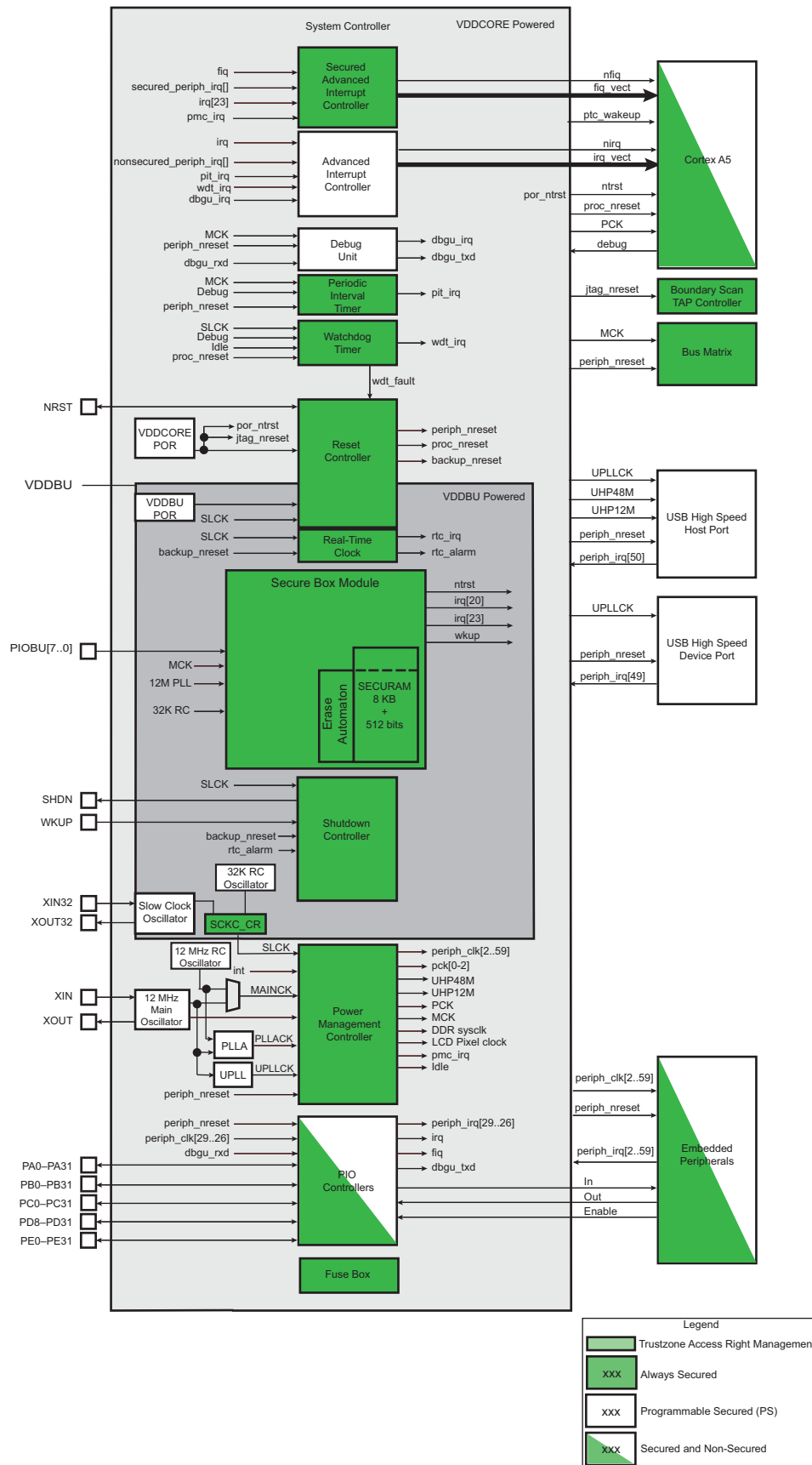
Figure 7-1. SAMA5D4 System Controller Block Diagram
