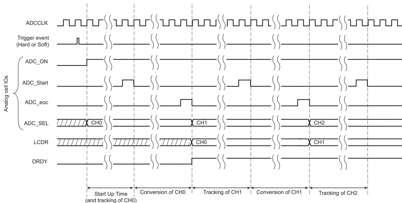
Figure 47-2. Sequence of ADC Conversions
