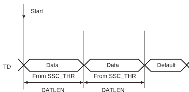
Figure 40-17. Transmit Frame Format in Continuous Mode (STTDLY = 0)
