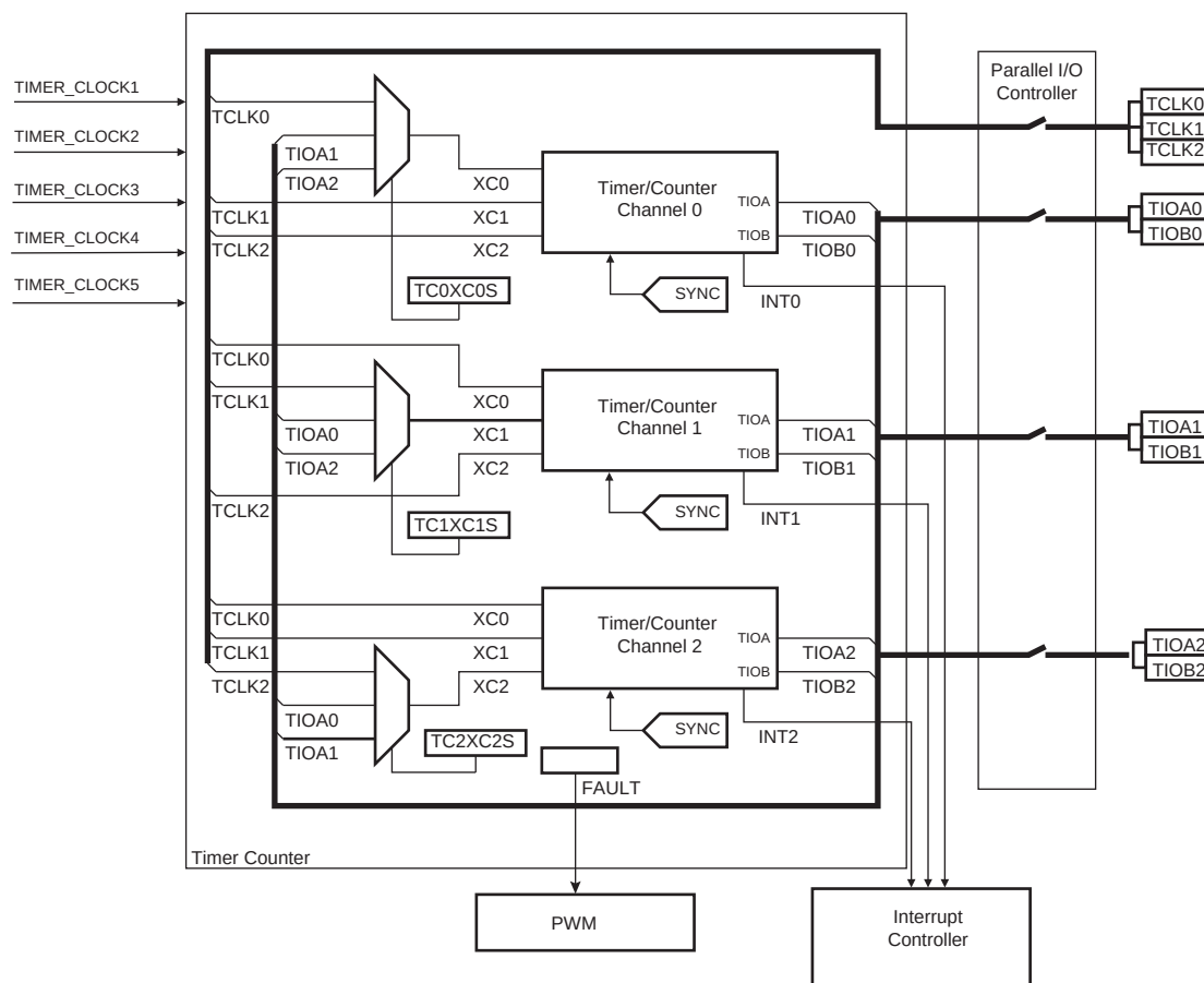
Figure 45-1. Timer Counter Block Diagram
