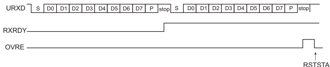
Figure 42-4. Character Reception
