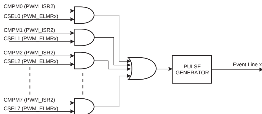
Figure 46-17. Event Line Block Diagram
