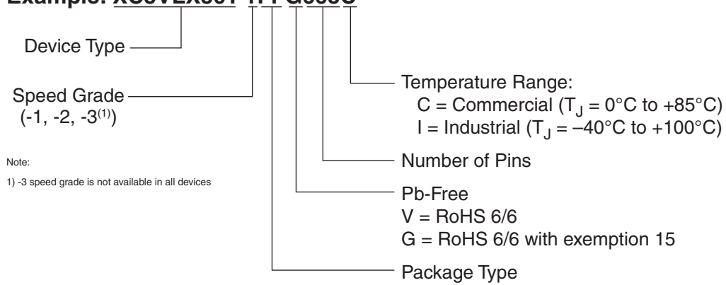
Figure 1: Virtex-5 FPGA Ordering Information
