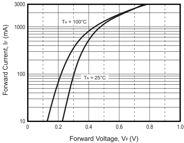
Fig.7 - Forward Characteristics
