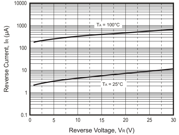
Fig.6 - Reverse Characteristics
