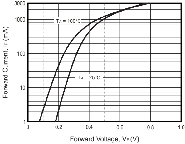
Fig.5 - Forward Characteristics
