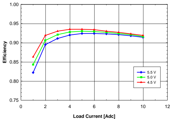
Fig. 1.8V.3: Efficiency vs. load current and input voltage for V_{out} = 1.8V converter mounted vertically with air flowing from pin 10 to pin 1 at a rate of 200 LFM (1m/s) and T_a = 25^{\circ}\text{C} .
