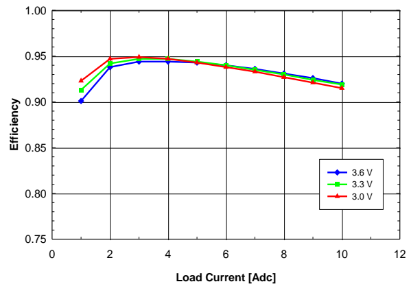
Fig. 1.8V.4: Efficiency vs. load current and input voltage for V_{out} = 1.8V converter mounted vertically with air flowing from pin 10 to pin 1 at a rate of 200 LFM (1m/s) and T_a = 25^{\circ}\text{C} .
