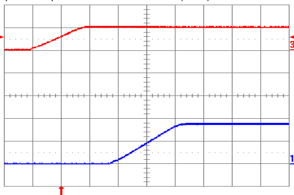
Fig. 1.8V.5: Turn-on transient for V_{out} = 1.8V with application of V_{in} at full rated load current (resistive) and 47\mu\text{F} external capacitance at V_{in} = 5V . Top trace: V_{in} (5V/div.); Bottom trace: output voltage (1V/div.); Time scale: 2ms/div.
