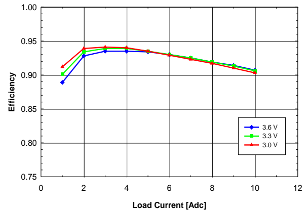
Fig. 1.5V.4: Efficiency vs. load current and input voltage for V_{out} = 1.5V converter mounted horizontally with air flowing from pin 10 to pin 1 at a rate of 200 LFM (1m/s) and T_a = 25^\circ C .
