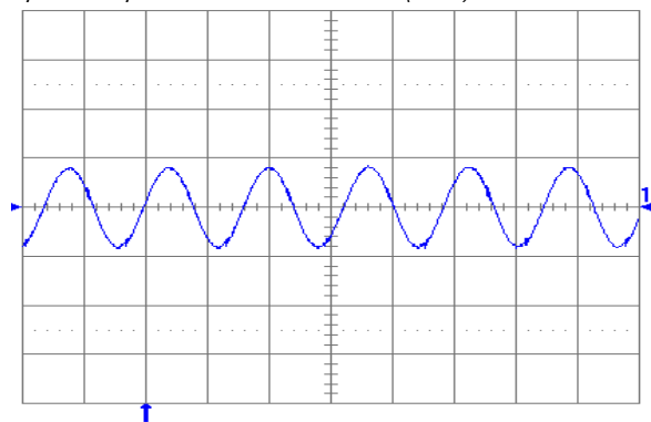
Fig. 1.8V.6: Output voltage ripple (20mV/div.) at full rated load current into a resistive load with external capacitance 47\mu\text{F} ceramic + 1\mu\text{F} ceramic and V_{in} = 5V for V_{out} = 1.8V . Time scale: 2µs/div.
