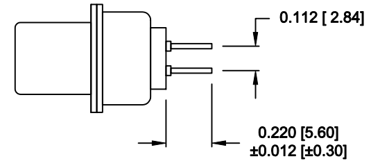
SIGNAL CONTACTS
