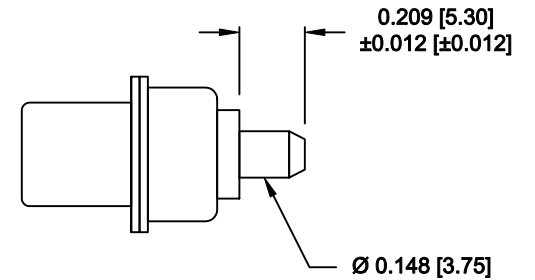
POWER CONTACTS
