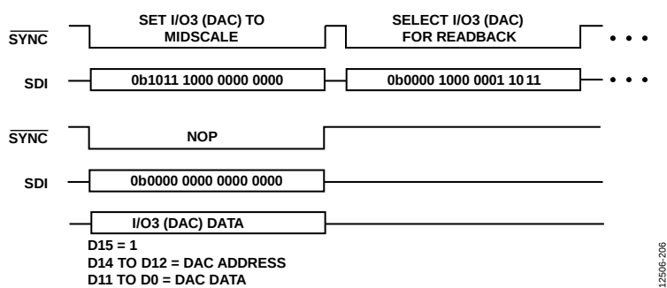
Figure 41. DAC Readback Operation
