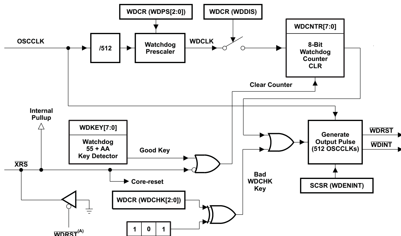
Figure 3-13. Watchdog Module
