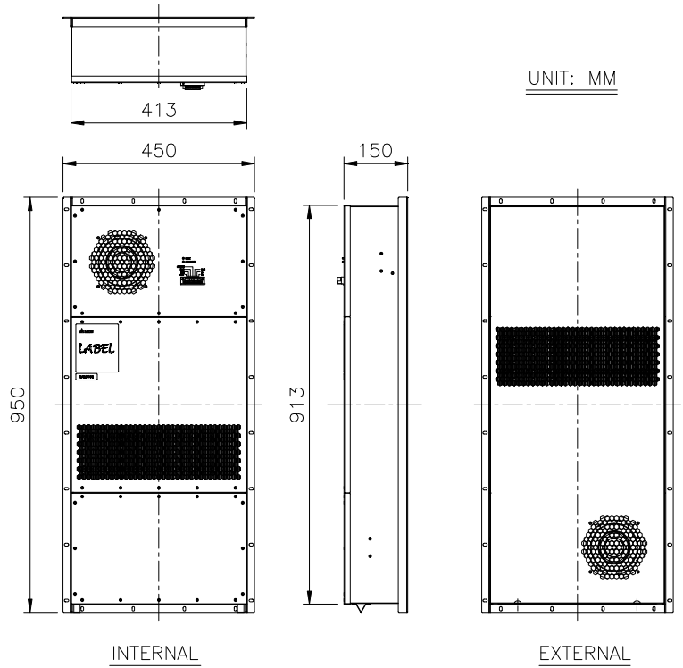
Dimension drawing
