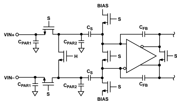
Figure 26. Switched-Capacitor Input
