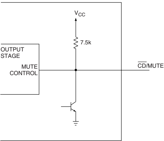
Figure 5 \overline{CD}/MUTE Circuit
