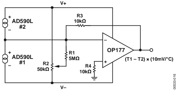
Figure 19. Differential Measurements
