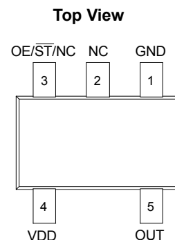
Figure 1. Pin Assignments
