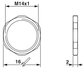
Dimensional drawing
