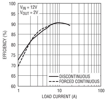
Efficiency vs Load Current with DCR Sensing
